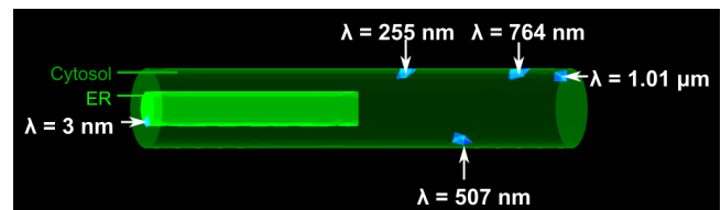
Figure 4: Simulation protocol for simulating neuronal stimulation at various ER-synapse distances with constant branchlet volume. IP 3 was infused in various tetrahedra (blue) in the 'Cyl_{1000} geometry (see Fig 1 and Table 1), located at various distances from the closest ER triangle, resulting in ER-synapse distances \lambda = 3, 255, 507, 764 and 1010 nm. The 'Cyl_{1000} geometry is a cylinder of length l_{\text{cyt}} = 2 \mu\text{m} .
