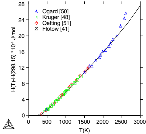
Fig. 6. Calculated enthalpy increment versus temperature for PuO 2 (present work, SGTE, 42) – comparison with the experimental data.
