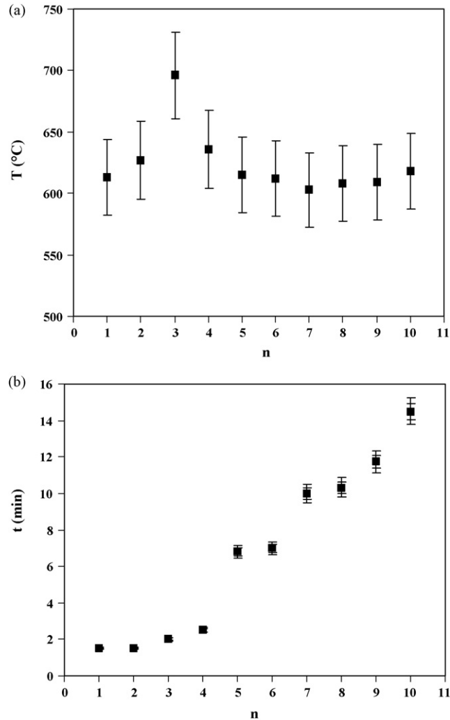
Fig. 1. Temperature reached by the furnace during combustion in a furnace pre-heated at 600 ^{\circ}\text{C} (a) and time for completion of reaction (b) vs. the proportion of urea ( n ) used for the combustion synthesis.
