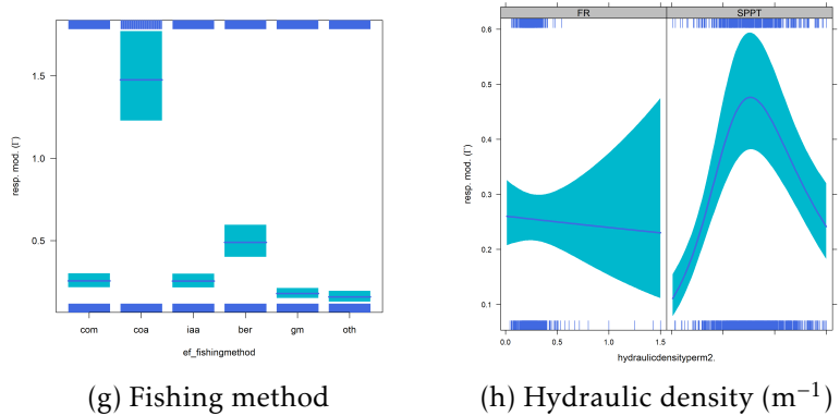
Figure 3.12: Predictors of the \Gamma model. (a) (b) two dimensional contour plot to show the interaction, (c)-(h) Response plot, the values in the Y-axis correspond to densities ( eel.m^{-2} ) for the \Gamma model (modelled on a subset of positive values). When not included in the plots, variables have been set to: cumulated height dam ^{10} = 0 m, altitude = 0 m, distance sea = 0 km, distance to Gibraltar = 3000 km, fishing method = full (two pass wadable electrofishing \omega_{ful} ), year=2015.
