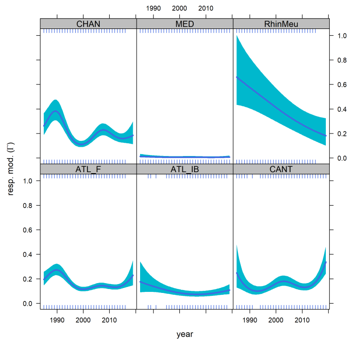
(a) Year:area_sudo
