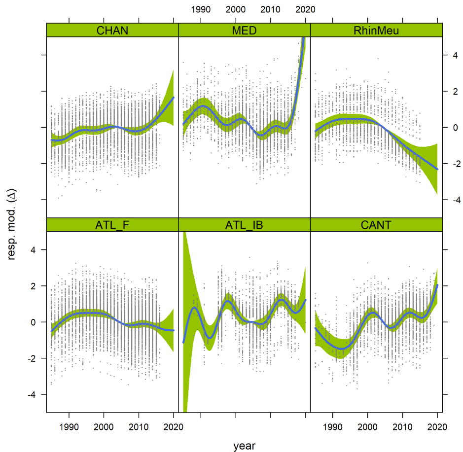
Figure 3.9: Response of the \Delta model for year. A different response has been obtained for the different SUDOE areas. Data are missing after 2018 in France so the trends of common areas (CANT and the MED) are probably biased after 2018. The level of the response per SUDOE area is provided in Figure 3.8e.
