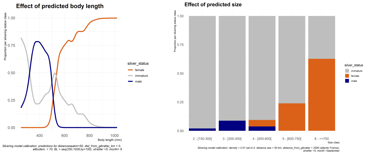
(a) Silver eel model - Body length
