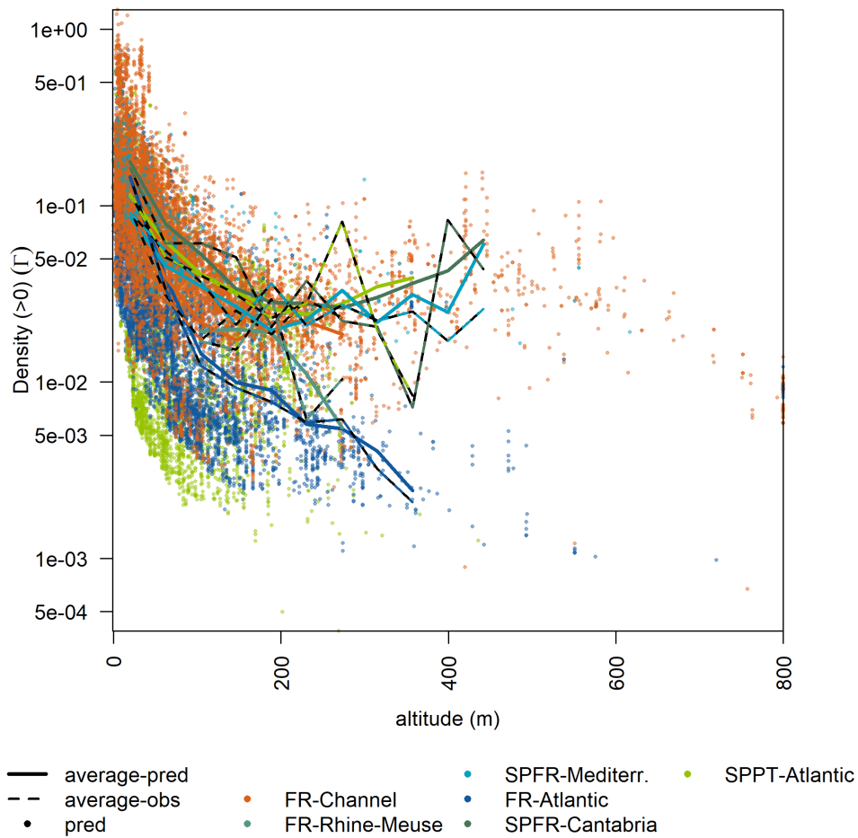
Figure 5.10: \Gamma model response for altitude.
