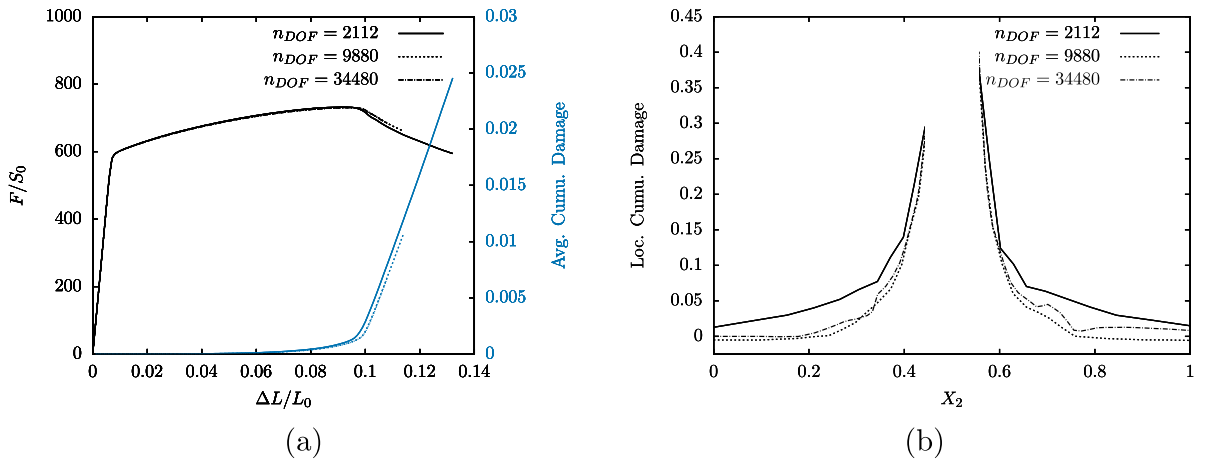
Fig. B.17. Mesh size convergence analysis on [100] – [010] – [001] crystal orientation in terms of (a) macroscopic stress–strain and average cumulated damage measures and (b) local cumulated damage at \Delta L/L_0 = 0.1 when acceleration of average cumulated damage sets on. H_\chi is set to 10^4 MPa. (For interpretation of the references to color in this figure legend, the reader is referred to the web version of this article.)
