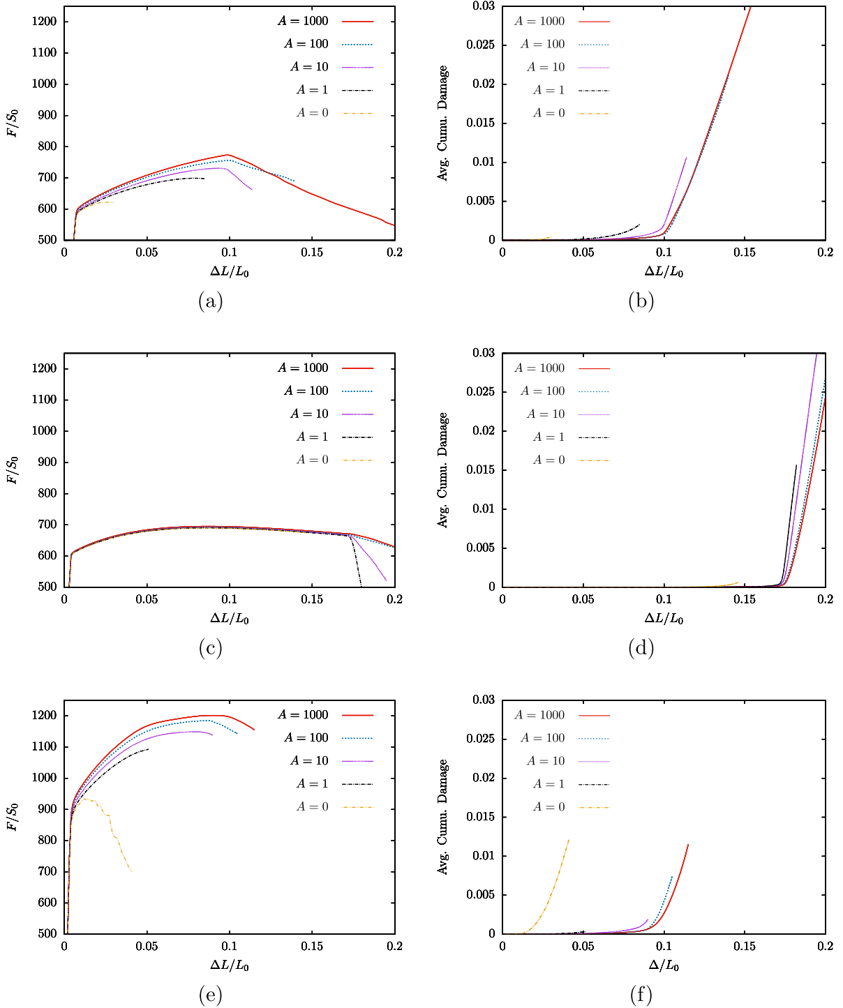
Fig. 4. Influence of parameter A on macroscopic stress–strain and average cumulated damage curves for crystal directions ([100],[010],[001]) in (a–b), ([110],[\bar{1}\bar{1}0],[001]) in (c–d) and ([111],[\bar{2}11],[0\bar{1}\bar{1}]) in (e–f). H_\chi is set to 10^4 MPa.
