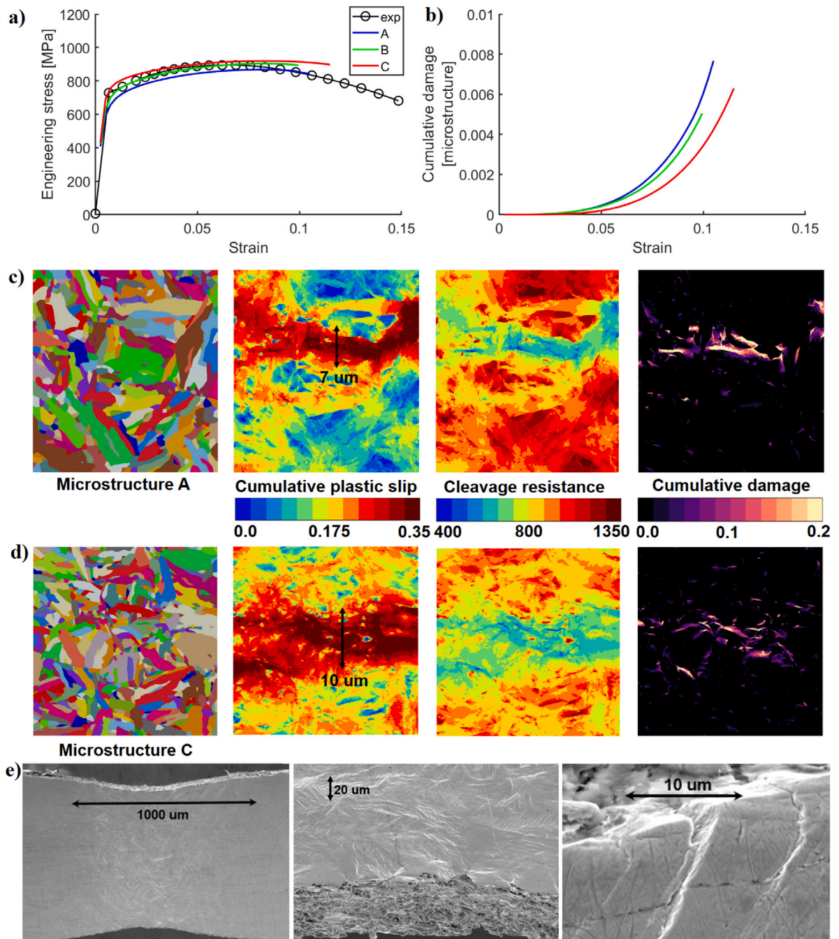
Fig. 13. (a) Experimental and simulated stress–strain curves, (b) simulated cumulative damage over the whole microstructure, (c) and (d) microstructure, cumulative plastic, effective cleavage resistance, and cumulative damage for microstructures A ( \epsilon = 10.5\% ) and C ( \epsilon = 11.5\% ), respectively. (e) SEM characterization of a small-scale tensile specimen with strain localization and cracking.
