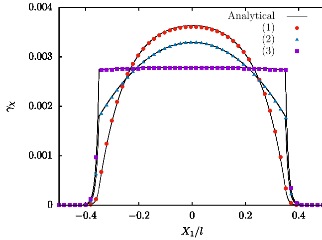
Fig. A.15. Analytical (solid lines) and numerically computed (colored dots) profiles of micro-slip in the periodic two-phase laminate at 0.2% macroscopic shear strain obtained with the micromorphic model with material parameters presented in Table A.3. (1) in absence of mismatch of the characteristic length between the two phases A^s = A^h = 5 \times 10^{-5} MPa mm 2 , (2) an intermediate mismatch between the two phases A^s = 1 \times 10^{-3} MPa mm 2 and A^h = 5 \times 10^{-5} MPa mm 2 , (3) a stronger mismatch between the two phases A^s = 5 \times 10^{-2} MPa mm 2 and A^h = 5 \times 10^{-5} MPa mm 2 . The fraction of soft phase is f_s = 0.7 and the microstructure size \ell = 1 \mu\text{m} .
