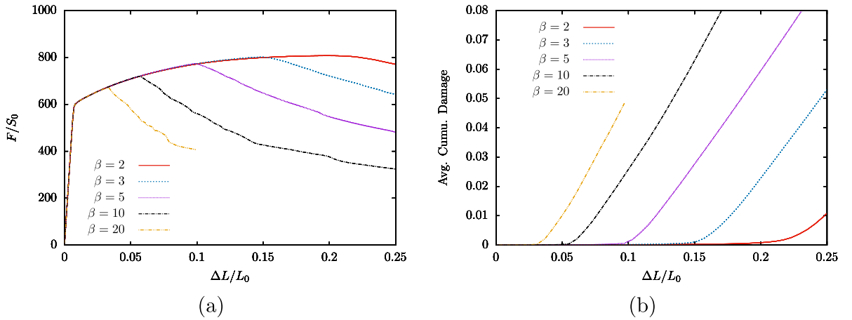
Fig. C.18. Influence of parameter \beta on (a) the stress–strain behavior and (b) average cumulated damage evolution for a [100]–[010]–[001] crystal orientation with H_\gamma = 10^4 MPa.
