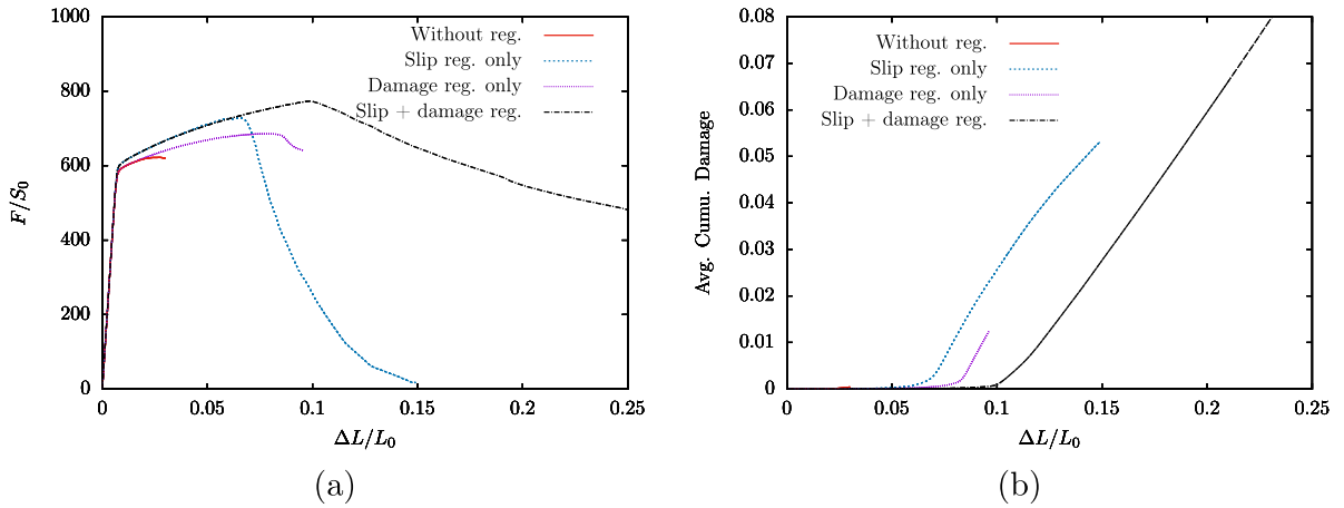
Fig. 2. Influence of the chosen variable for gradient regularization on (a) the stress–strain behavior and (b) average cumulated damage evolution for a [100] - [010] - [001] crystal orientation. H_\chi is set to 10^4 MPa.
