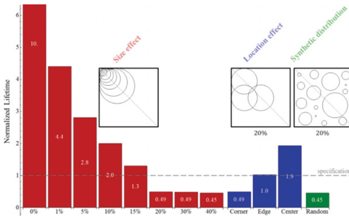
Figure 2. Lifetime normalized with respect to specification of 10000 cycles for different configurations of voids.
