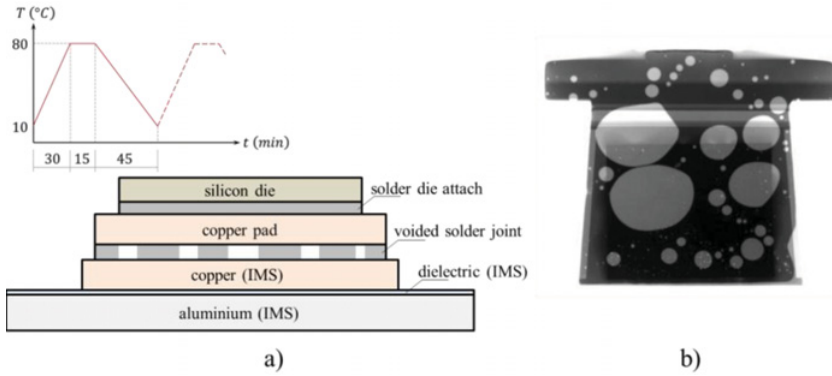
Figure 1. a) Schematic representation of the electronic assembly, b) X-ray tomography inspection of the solder voids.
