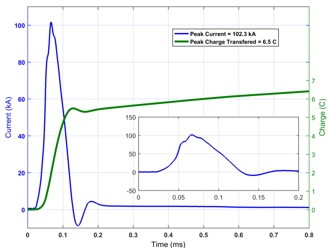
Fig. 2. Measured current (blue) and calculated transferred charge associated with the first return stroke of the flash. An expanded view of the current waveform is shown in the inset.
