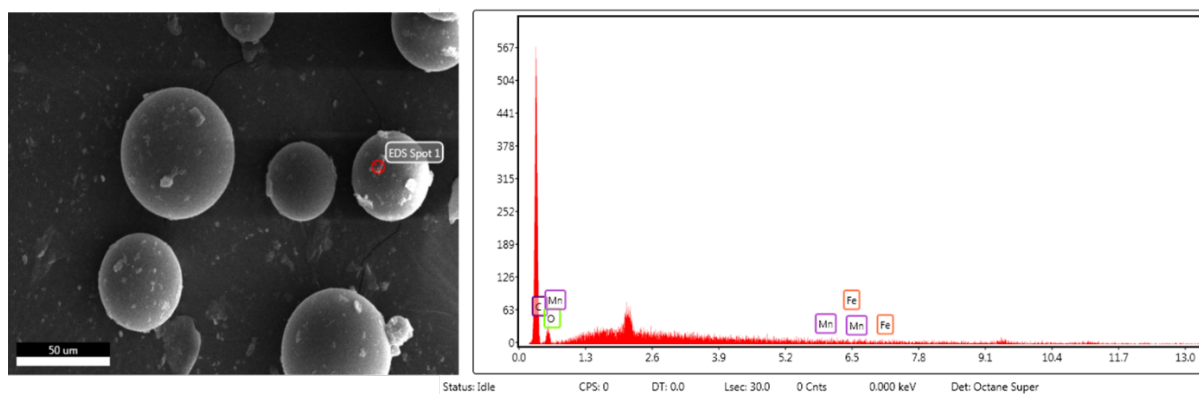
Fig. S9. SEM-EDX images of aged PS-MP.
