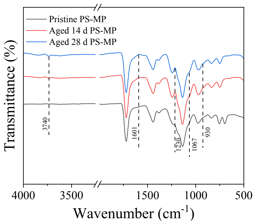
Fig. S10. ATR-FTIR spectra of PS-MP aging for different times, i.e., 0, 14 and 28 days.
