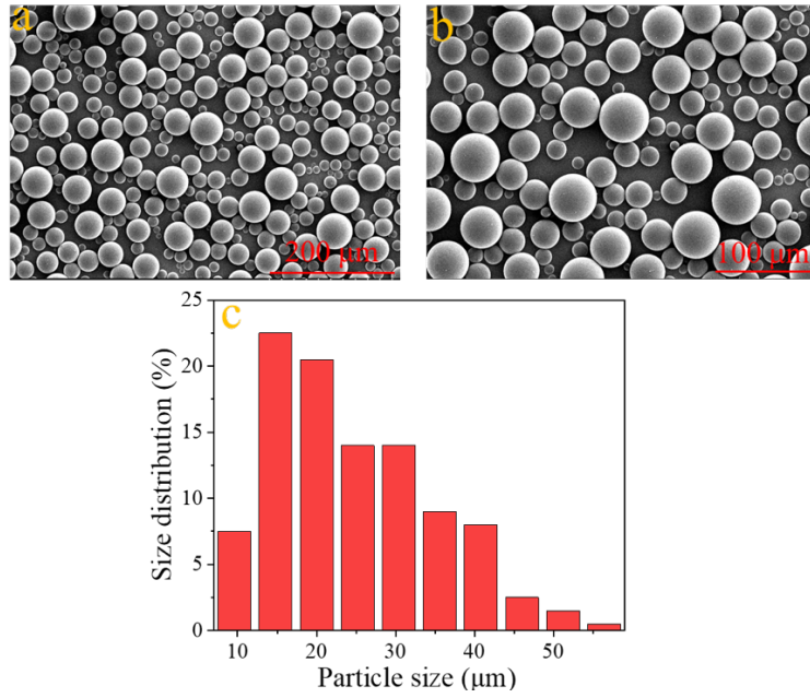
Fig. S1. Scanning electron microscope (SEM) images for PS-MP and particle size analyze using Nano measure 1.2
