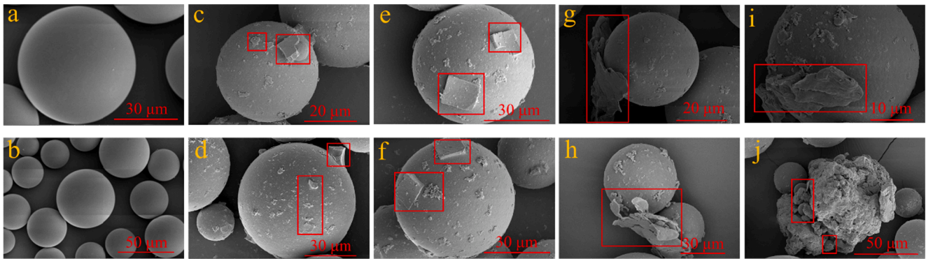
Fig. 8. SEM images of pristine (a, b), aging for 7 days (c, d), 14 days (e, f), 21 days (g, h) and 28 days (i, j) polystyrene microplastic (PS-MP) particles. The morphology of PS-MP changed from smooth to rough with aging, indicating PS-MP was wrapped by soil particles to form the protective layer.
