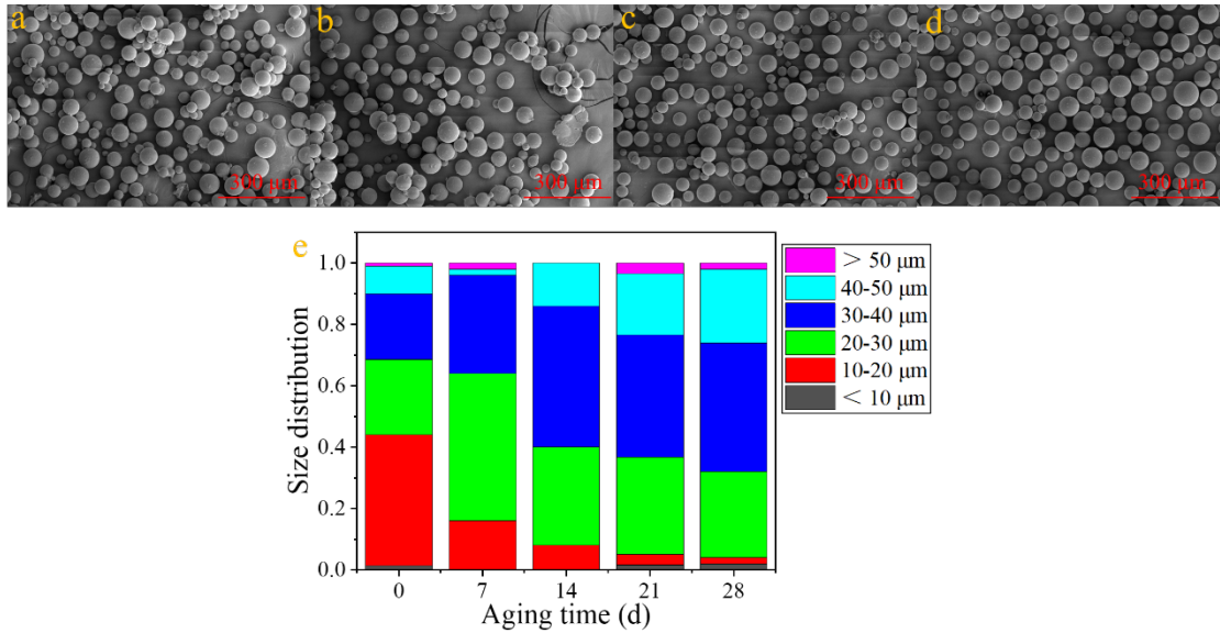
Fig. S11. SEM images of PS-MP aged for 7 days (a), 14 days (b), 21 days (c) and 28 days (d), and the size distribution of PS-MP with different aging times (e). All particles in the SEM images were measured by using a Nano Measurer to obtain the size distribution.
