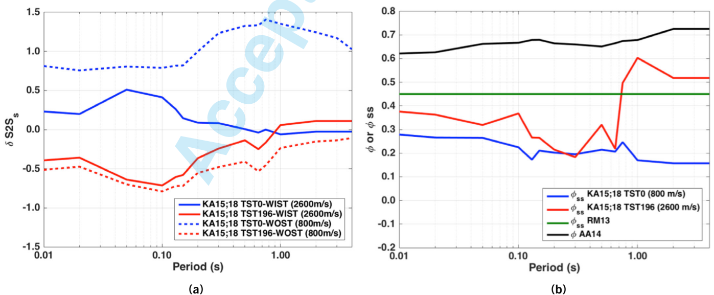
Fig. 6 - Site-specific residuals calculated at stations TST_0 and TST_{196} by Ktenidou et al., 2015a, 2018 (KA15;18) with respect to the AA14 GMPE (Akkar et al., 2014): (a) site terms \delta S2S_s , estimated for stations TST_0 (blue) and TST_{196} (red) with the AA14 site term accounting for V_{S30} (WIST, solid lines), or without the site term, i.e., with respect to standard rock 800m/s (WOST, dotted lines). (b) Standard deviation of the within-event term ( \phi ) and standard deviation of the site specific within-event residual term ( \phi_{SS} ).
