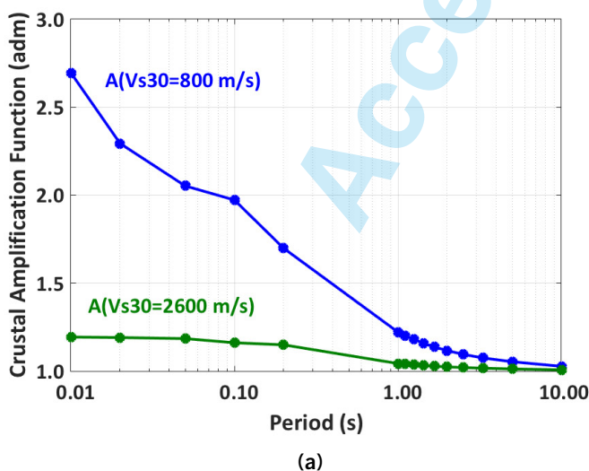
Fig. 3 - Rock to hard rock corrections for TST site at Euroseistest. (a) Crustal amplification functions for a standard rock site ( V_s=800 m/s, blue) and for a hard-rock site ( V_s=2,600 m/s, green). (b) The Shear Wave Velocity Correction (VSC) corresponding to the ratio between these two quarter-wavelength crustal amplification functions.
