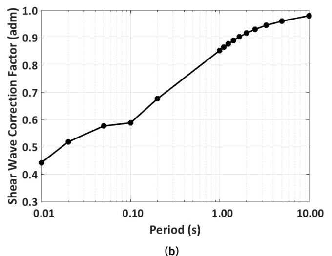
Fig. 3 - Rock to hard rock corrections for TST site at Euroseistest. (a) Crustal amplification functions for a standard rock site ( V_s=800 m/s, blue) and for a hard-rock site ( V_s=2,600 m/s, green). (b) The Shear Wave Velocity Correction (VSC) corresponding to the ratio between these two quarter-wavelength crustal amplification functions.
