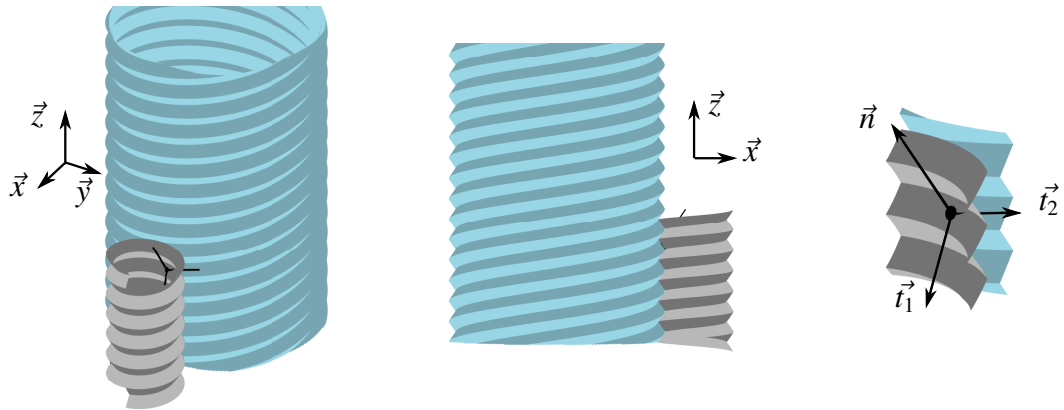
Figure 5: a. 3D view of the roller-screw contact. b. Normal view of the contact with tangency between the dark grey and dark blue surfaces. c. Zoom on a contact with normal vector \vec{n} and pair of tangent vectors (\vec{t}_1, \vec{t}_2) given by Hertz main directions.
