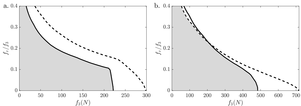
Figure 11: Mechanism fatigue analysis. a. Standard PRS (example 1) and b. Inverted PRS (example 2) under normal loading f_3 and relative tangential loading f_v/f_3 . Sliding coefficient is chosen as \epsilon = \epsilon^* . Solid lines correspond to roller-screw contact and dashed lines correspond to roller-nut contact. Grey areas correspond to infinite life domains of the mechanism.
