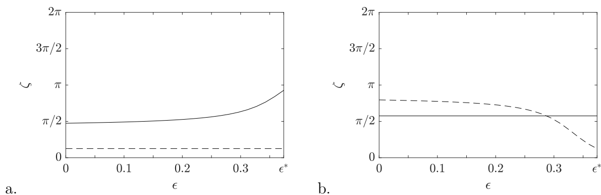
Figure 15: Hertz sliding angle \zeta dependence on sliding coefficient \epsilon in a. standard PRS (example 1) and b. inverted PRS (example 2). Solid line corresponds to Roller-Screw contact and dashed line corresponds to Roller-Nut contact.
