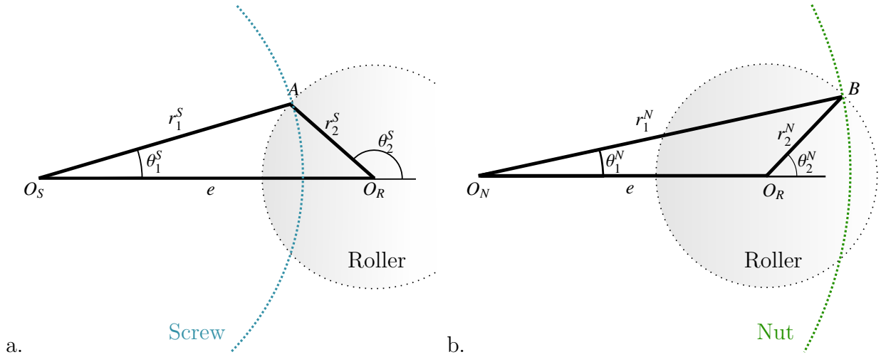
Figure 6: Contacts points between a. screw and roller (A) and b. nut and roller (B). O_S is the center of the screw ; O_N is the center of the nut ; O_R is the center of the roller.
