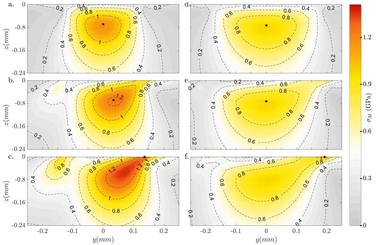
Figure 9: Color map of Von Mises stress \sigma_M for example 1 (standard PRS) with normal ( f_3 = 100N ) and tangential (in \vec{t}_2 , corresponding here to y -direction) loads. Left column: roller-screw contact (maximal Hertz pressure = 1.87 GPa); Right column: roller-nut contact (maximal Hertz pressure = 1.56 GPa). a and d, \mu = 0 ; b and e, \mu = 0.25 , c and f, \mu = 0.4 . \star corresponds to the depth of the maximum stress z . Sliding coefficient is chosen as \epsilon = \epsilon^* , Eq. 13.
