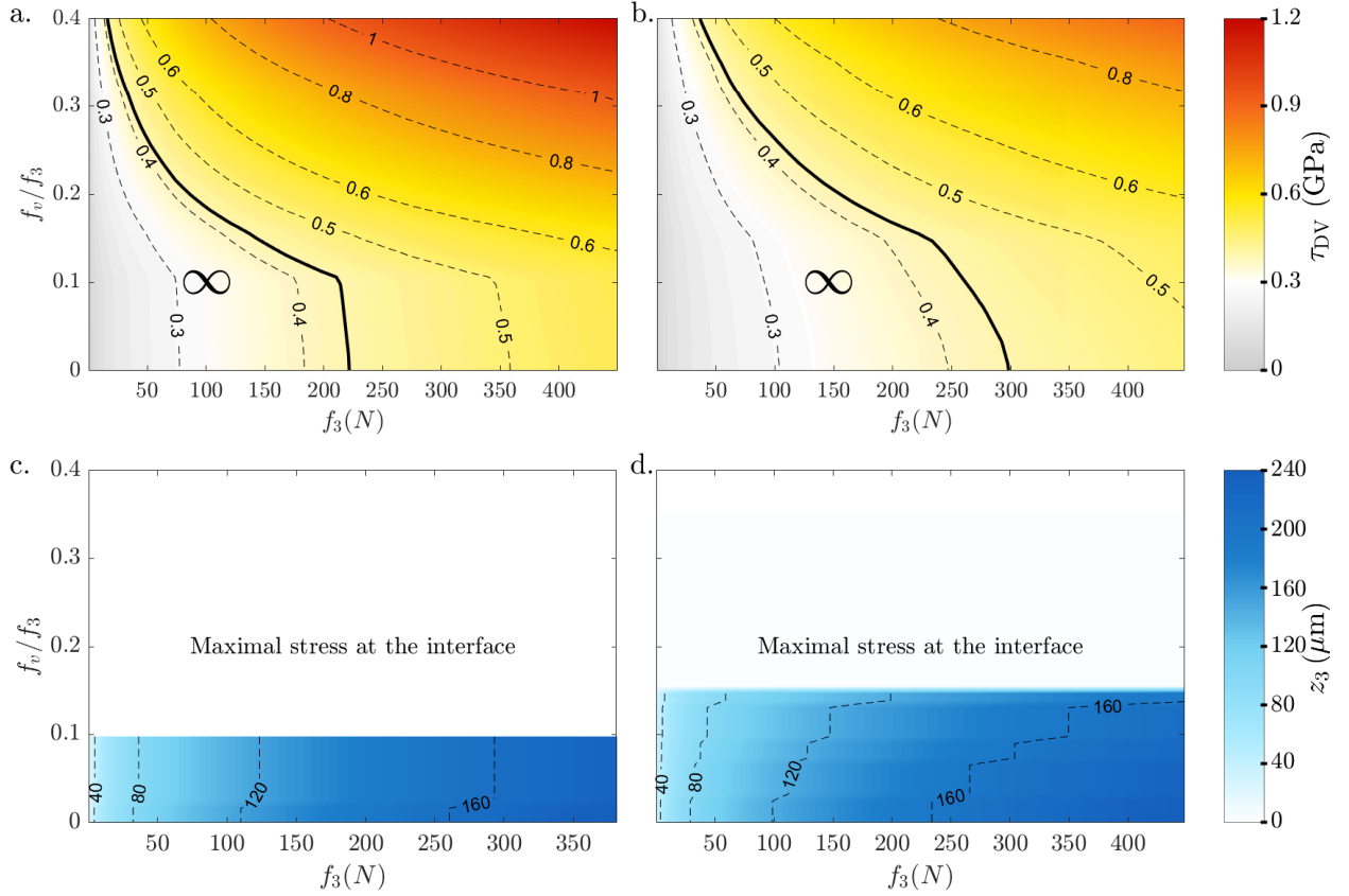
Figure 10: Fatigue analysis of example 1 (Standard PRS) under normal loading f_3 and relative tangential loading f_v/f_3 . Sliding coefficient is chosen as \epsilon = \epsilon^* , Eq. 13. Color map of Dang Van stress \tau_{DV} for a. roller-screw contact and b. roller-nut contact. Solid line separates infinite PRS life domain (left, corresponding to small normal loads) from finite life domain (right, corresponding to large normal loads). The solid line is given by \tau_{DV} = L_t , equation (21). Usual friction coefficient are small f_v/f_3 < 0.1 . Color maps of depth of maximal Dang Van criterion z_{max} for c. roller-screw contact and d. roller-nut contact.
