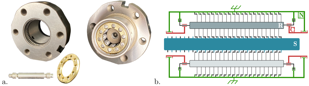
Figure 2: Standard PRS mechanism. a. Photo of each component (left) and assembled mechanism (right) b. Kinematic diagram of a standard PRS mechanism. The nut (green) is in thread and gear contact with the rollers (grey). The rollers and the screw (blue) are in thread contact. The carriers are in sliding pivot link with the rollers and pivot link with the nut.
