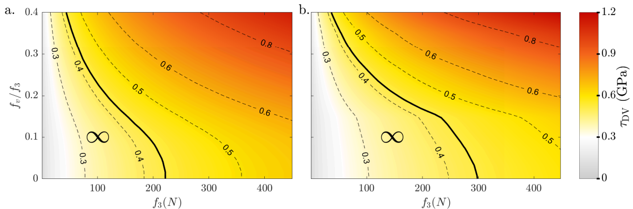
Figure 13: Fatigue analysis of example 1 (Standard PRS) under normal loading f_3 and relative tangential loading f_v/f_3 . Sliding coefficient is chosen as \epsilon = 0 . Dang Van stress \tau_{DV} for a. roller-screw contact and b. roller-nut contact. Solid line separates infinite PRS life domain (left, corresponding to small normal loads) from finite life domain (right, corresponding to large normal loads). Classically, for steels, friction coefficient is in the order of f_v/f_3 \approx 0.1 .
