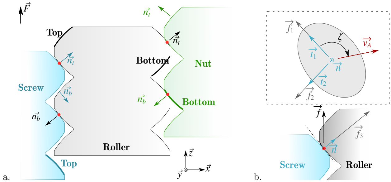
Figure 4: a. Definition of the orientation of the contact normals. b. Contact frame of reference. Definition of sliding velocity at the contact \vec{v}_A and Hertz sliding angle \zeta .
