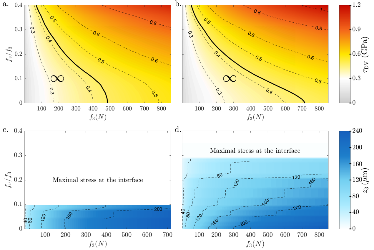
Figure 12: Fatigue analysis of example 2 (Inverted PRS) under normal loading f_3 and relative tangential loading f_v/f_3 . Sliding coefficient is chosen as \epsilon = \epsilon^* , Eq. (14). Dang Van stress \tau_{DV} for a. roller-screw contact and b. roller-nut contact. Solid line separates infinite PRS life domain (left, corresponding to small normal loads) from finite life domain (right, corresponding to large normal loads). Classically, for steels, friction coefficient is in the order of f_v/f_3 \approx 0.1 . Color maps of depth of maximal Dang Van criterion z_{max} for c. roller-screw contact and d. roller-nut contact.
