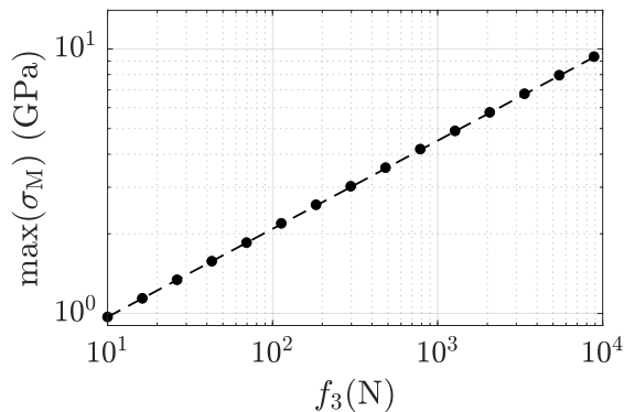
Figure 7: Hertz contact scaling of maximal Von Mises Stress \max(\sigma_M) as a function of normal load f_3
