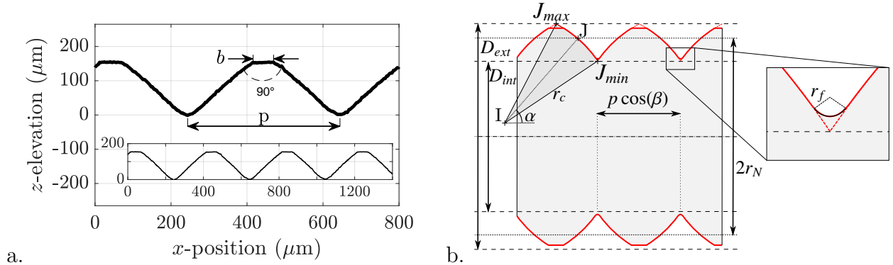
Figure 3: a. Screw thread cross section obtained by optical microscopy (STIL 3D measuring station). b. Notations and parameters of the threads. I is the centre of curvature . J is the point located on the profile and forming an angle \alpha = 45^\circ with the axis of revolution. ( J_{max} and J_{min} are boundaries of the mathematical profile).
