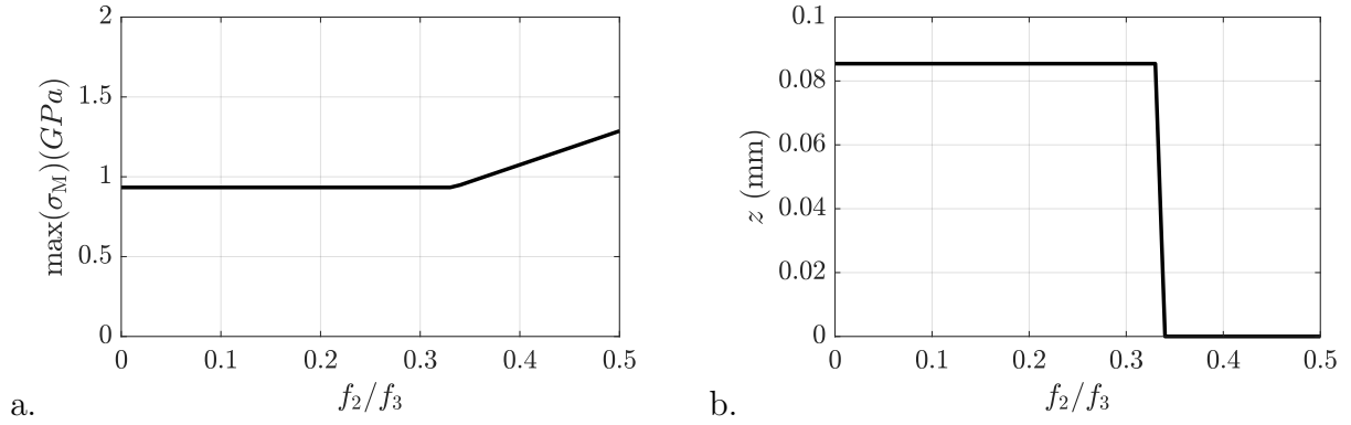
Figure 8: Standard PRS (example 1) under relative tangential loading f_2/f_3 . a. Maximum Von Mises stress \sigma_M and b. depth of the maximum stress.
