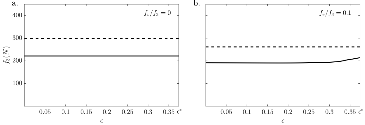
Figure 14: Standard PRS (example 1) under sliding coefficient and normal loading per contact f_3 . Relative tangential loading is chosen as a. f_v/f_3 = 0 and b. f_v/f_3 = 0.1 . Solid line corresponds to roller-screw contact and dashed line corresponds to roller-nut contact.
