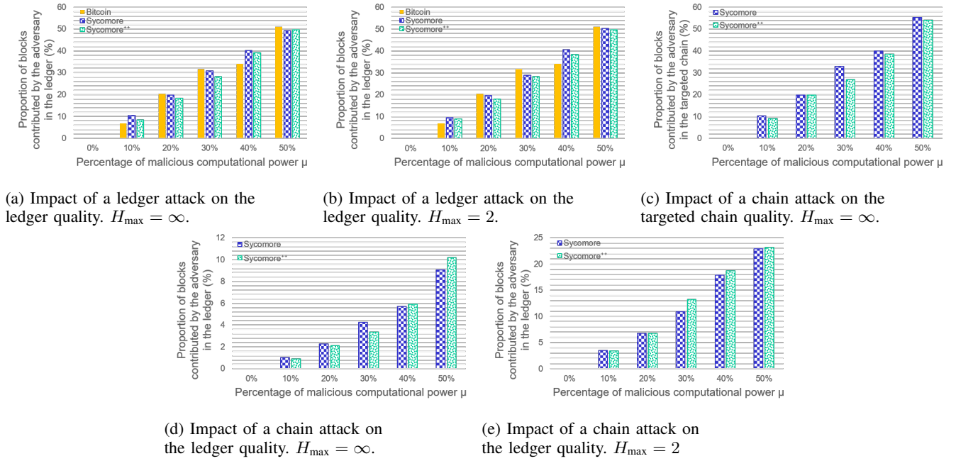
Fig. 3: Impact of the ledger and chain attacks
