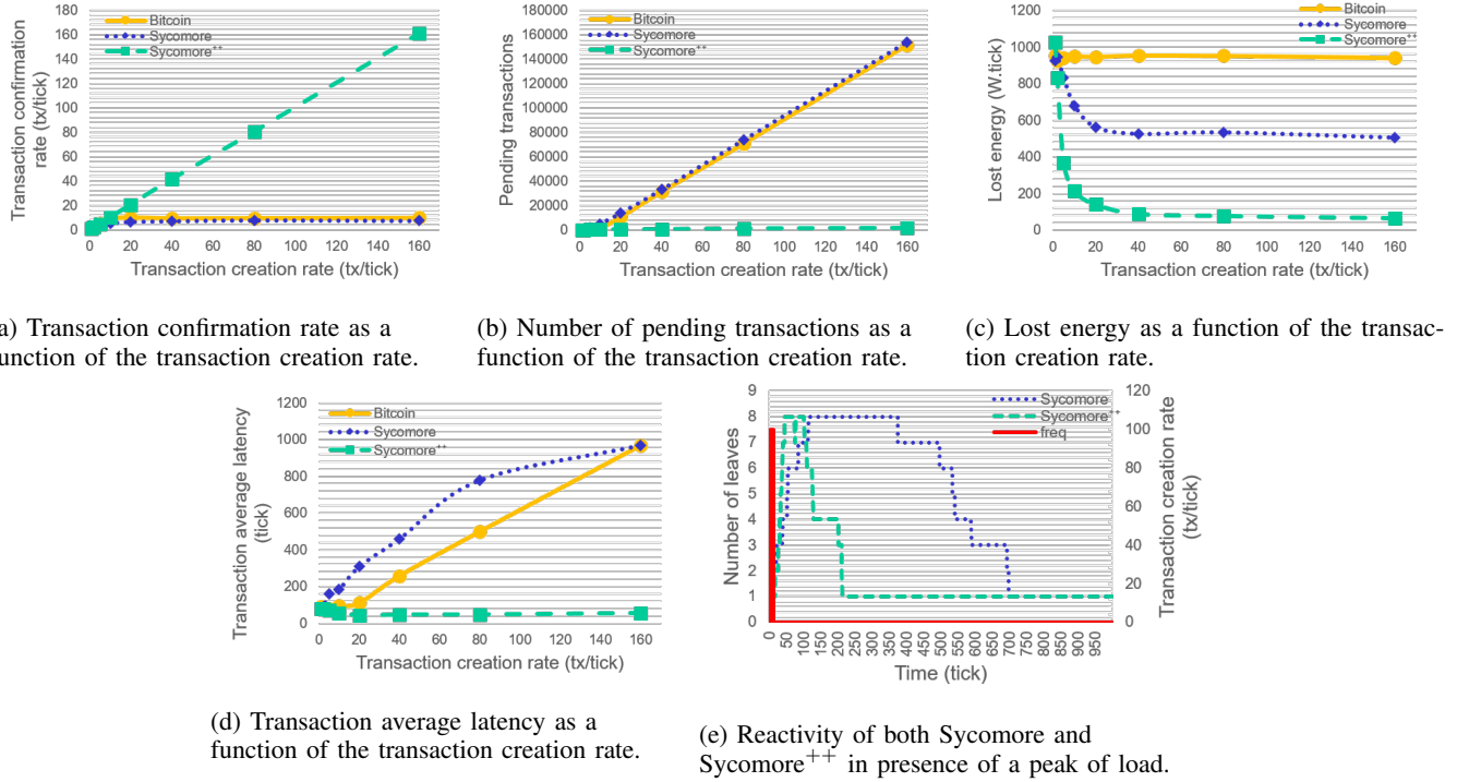
Fig. 2: Scalability of Bitcoin, Sycomore and Sycomore ++ (overload threshold \Gamma = 90\% , underload threshold \gamma = 0\% ) and Reactivity of both Sycomore and Sycomore ++ ( \Gamma = 90\% , \gamma = 10\% ).
