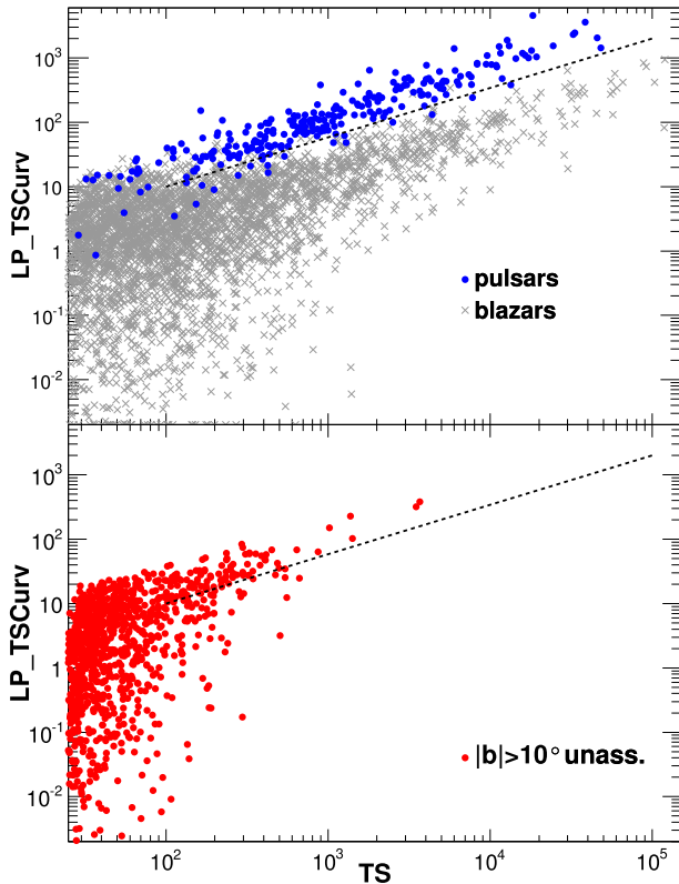
Figure 15. Top: parameter LP\_TS_{curv} (reflecting the spectral-curve significance) as a function of Test Statistic for blazars and pulsars (no selection on the Galactic latitude was applied). The dotted line, selected by eye, approximately delineates the separation between the two corresponding branches. Bottom: same for the high-latitude unassociated sources. The same dotted line as in the top panel is displayed for orientation.
