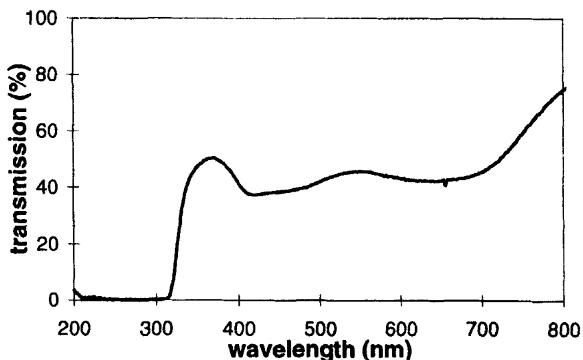
FIGURE 4 Transmitted light spectrum as a function of wavelength for the sandwich-cell after 25 min of annealing
