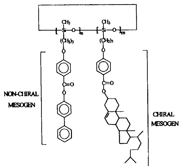
FIGURE 1 General chemical structure of CLC polysiloxanes
