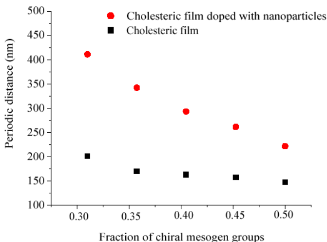
Figure 3. Periodic distance between lines (np ribbons) vs. the molar fraction in chiral mesogens present in the pure (doped) cholesteric host.
