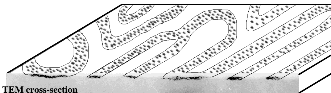
Fig. 3. A possible sketch of np ribbons from the film plane to the cross-section.
