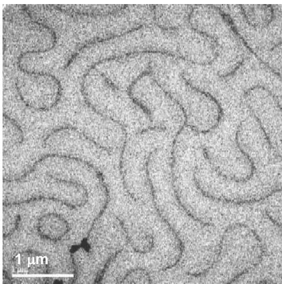
Fig. 1. TEM micrograph of cholesteric LC SR doped with np. Particle assemblies are structured into ribbons which mimic the fingerprint texture.
