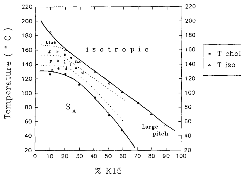
FIGURE 1 SB/K15 phase diagram. We have mentioned the qualitative variation of the pitch in the cholesteric region: selective reflections colours and large pitch zone.
