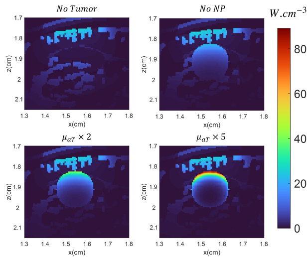
Fig. 5. Heat deposition rate Q_H in \text{W.cm}^{-3} in the four cases considered at 808 nm.
