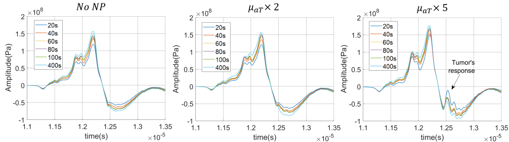
Fig. 11. Differential signal \Delta p(t) as PTT process progress for the three tumorous cases. Legend show how much time of PTT has passed in order to obtain the associated differential. The tumor's influence on the signal is indicated on the " \mu_{aT} \times 5 " case.
