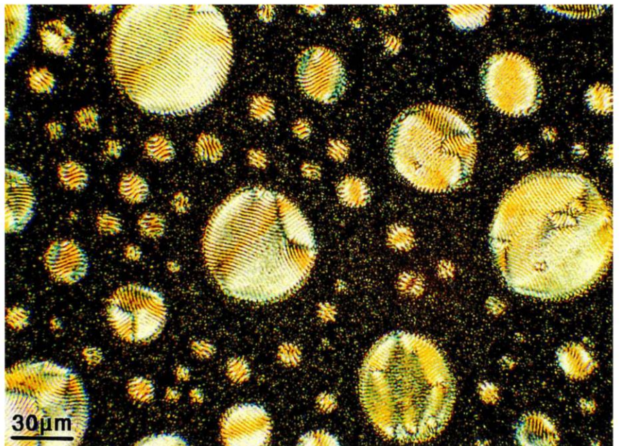
Figure 4. Cholesteric droplets embedded in the isotropic phase entrapped by UV polymerization (25°C).
