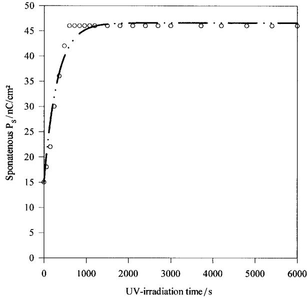
Figure 7. Spontaneous polarization as a function of the irradiation time for the slow curing process. The dashed curve corresponds to an approximate fit to equation (7 a).
