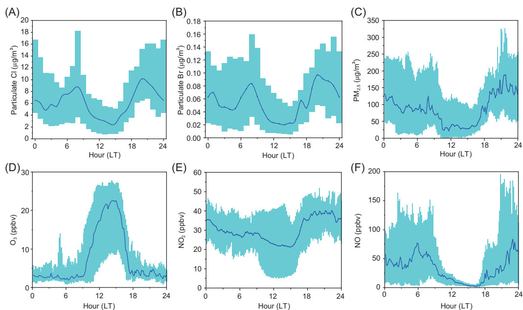
Figure 3. The observed diurnal profiles of trace gases and aerosol at the measurement site in NCP during 9–31 December 2017. (A) Particulate Cl, (B) particulate Br, (C) PM 2.5 , (D) O 3 , (E) NO 2 and (F) NO. The blue line is the median, and the cyan shade represents the 25 percentile and 75 percentile values.
