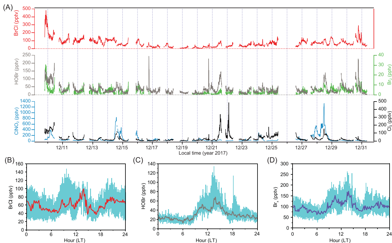
Figure 1. Ambient surface mixing ratios and diurnal profiles of reactive halogen gases at a rural site in NCP during 9–31 December 2017. (A) Time series of Cl 2 , ClNO 2 , HOBr, Br 2 and BrCl. (B) The diurnal profiles of BrCl for the entire period. The red line is the median, and the cyan shade represents the 25 percentile and 75 percentile values. (C) The diurnal profiles of HOBr for the entire period. The brown line is the median, and the cyan shade represents the 25 percentile and 75 percentile values. (D) The diurnal profiles of gas-phase bromine Br x (= BrCl + HOBr + 2 × Br 2 ) for the entire period. The purple line is the median, and the cyan shade represents the 25 percentile and 75 percentile values.
