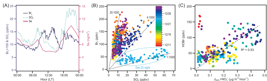
Figure 2. Evidence for the source of the observed reactive bromine gases: coal burning and photo-assisted activation process. (A) Average diurnal profile of Br_x (purple line in 10-min average), SO_2 (green dash line in 10-min average), and Se (red line in 1-hour average) during 9–31 December 2017. The lag in Br_x and its daytime peak are due to the photochemical release of Br_x from particulate matter. (B) Scatter plot of 10-min average Br_x and SO_2 from 18:00 to 09:00 when the air masses were stable. Color coded according to sampling date during 9–31 December 2017 ( Br_x = BrCl + HOBr + 2 \times Br_2 ). The dotted lines indicate Br_x/SO_2 slope (mole/mole) of 1 : 1000, 4 : 1000 and 20 : 1000, covering the range of Br_x production from coal burning. Data in the oval depict a case of industrial emissions. (C) Scatter plot of 10-min average HOBr and a proxy of photolysis rate of nitrate ( J_{NO_3^-} \times NO_3^- concentration) from 10:00 to 15:00. J_{NO_3^-} was calculated from the TUV model ( http://cprm.acom.ucar.edu/Models/TUV/Interactive_TUV ) under clear sky conditions and then scaled to the measured NO_2 photolysis rate coefficient ( J_{NO_2} ). Color coded according to sampling date during 9–31 December 2017. The outliers in the upper left corner are data from 2 days with the significant impact of fresh emissions or transport from the air aloft (Fig. S7).
