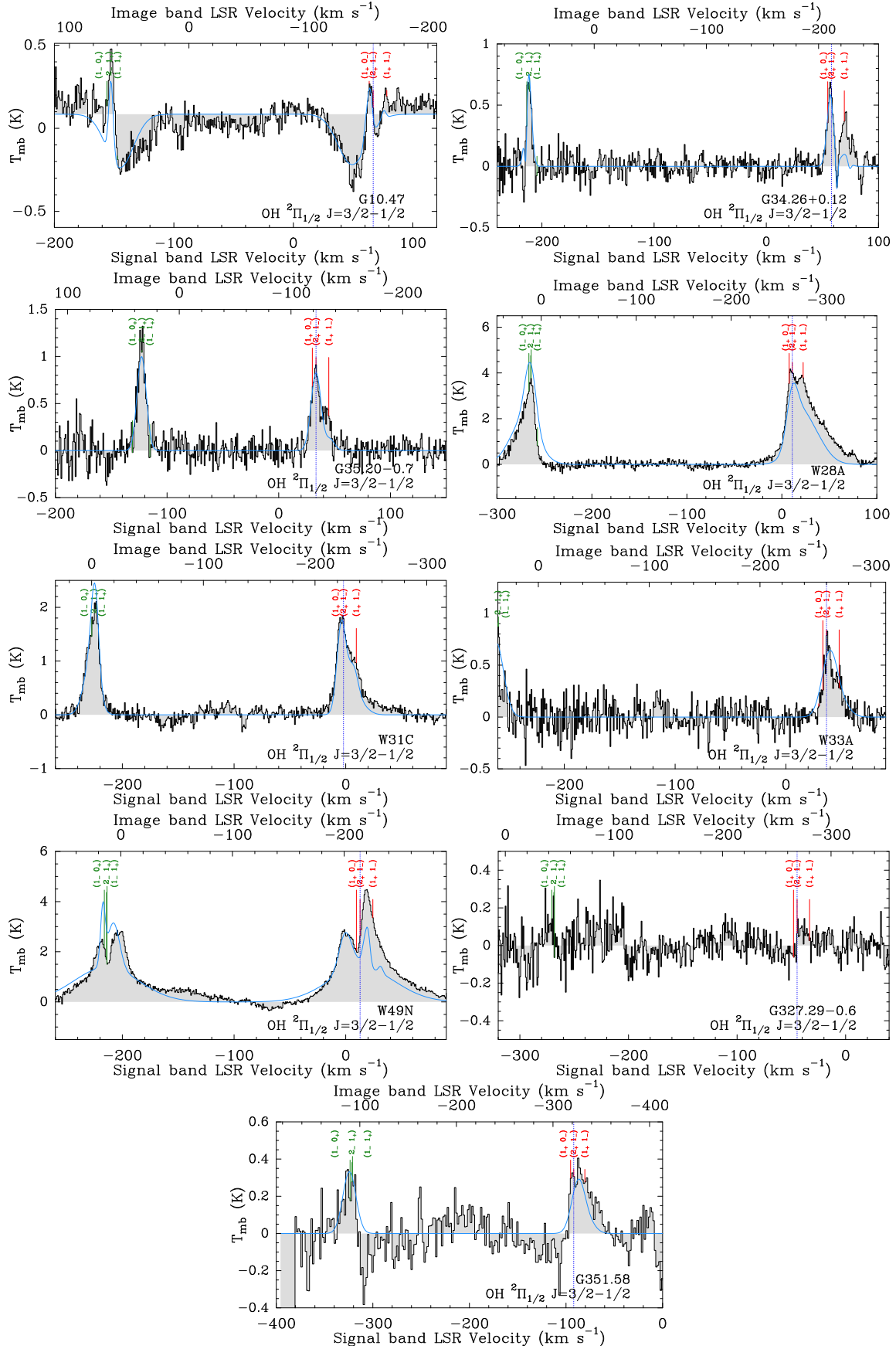
Fig. 4. Overview of OH ^2\Pi_{1/2} ( J = 3/2-1/2 ) transition towards the sample. The blue dotted line marks the systemic LSR velocity of the source in the signal band. The positions of the hfs lines are labelled in red in the signal and in green in the image band. The HFS fit to the spectra is shown in light blue. The velocity resolution is 0.75 \text{ km s}^{-1} for all sources, except for G351.58–0.4, where we show the spectrum at a velocity resolution of 1.5 \text{ km s}^{-1} .
