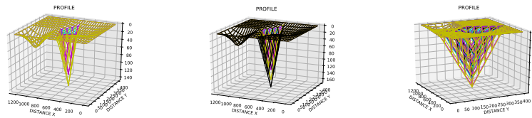
Figure 9: 2D profile optimization with limited capacity C = 1e6 , for T = 2, 3 and 6 time-frames.
