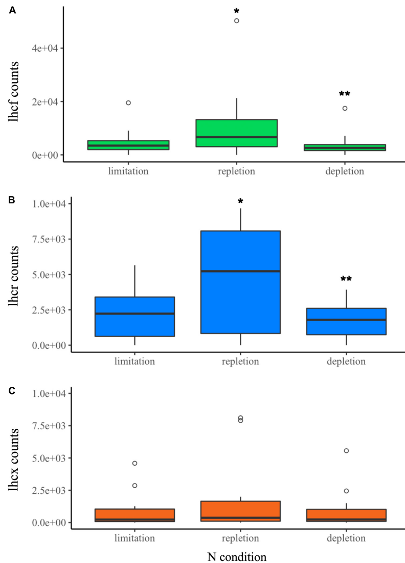
FIGURE 5 | CL experiment. Normalized transcript counts of (A) lhc f (green), (B) lhc r (blue), (C) lhc x (orange) genes according to N status (limitation, repletion, and depletion). Analysis of variance (ANOVA) test: * p -value < 0.05, ** p -value < 0.01.
