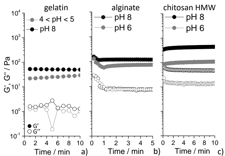
Figure S 1 – Time-dependence of G' and G'' (LVER, f=1 Hz, \gamma=0.1 %) for a) gelatin (2 wt%), b) alginate (1 wt% [ \text{Ca}^{2+} ]= 25 mM) and c) chitosan HMW (1 wt%) control hydrogels at basic and acidic pH. Values of pH are given on top of each panel.
