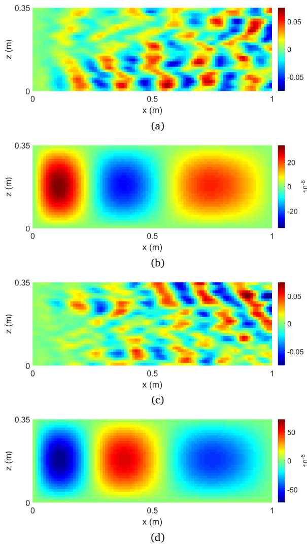
Figure 14: (a), (c): pressure fields (Pa) at the nodes of the spatial grid, generated by the C-UWPW method and (b), (d): their respective corresponding velocity fields (m/s), for a resonance (159 Hz).
