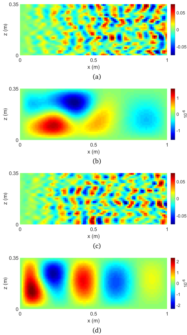
Figure 15: (a), (c): pressure fields (Pa) at the nodes of the spatial grid, generated by the C-UWPW method and (b), (d): their respective corresponding velocity fields (m/s), for an anti-resonance (277 Hz).
