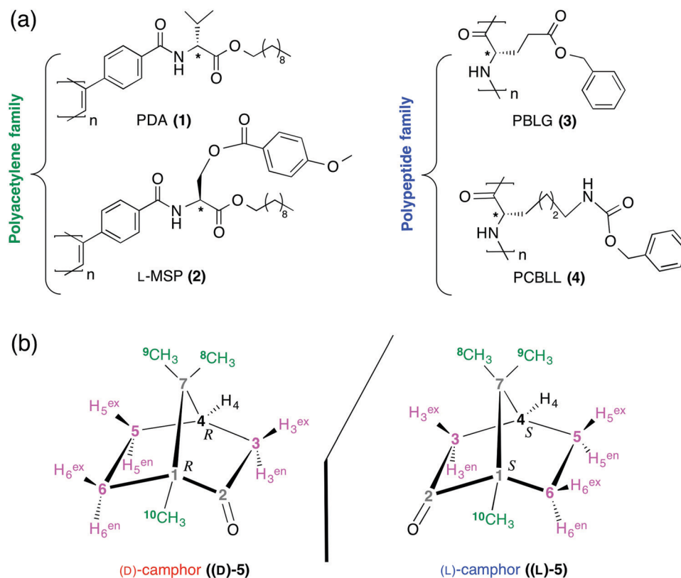
Fig. 1 (a) Structure of the four helical polymers investigated: PDA (poly- 1 ), L-MSP (poly- 2 ), PBLG (poly- 3 ), PCBL (poly- 4 ). Note the difference in the position of the stereogenic center; (b) structure of (D)-(1 R ,4 R )-(+)-camphor and (L)-(1 S ,4 S )-(–)-camphor ( 5 ) including their atomic numbering; the red and blue colors are used for identifying them. All ^1\text{H}/^2\text{H} NMR data related to the methyl, methylene ( \text{sp}^3 ) and methine ( \text{sp}^3 ) groups are identified by the green, pink and black colors, respectively.
