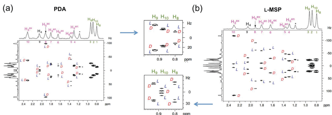
Fig. 2 92.1 MHz NAD- \{^1\text{H}\} Q -resolved Fz 2D spectrum (tilted and symmetrized) of 5 (ee( D ) = 30%) in (a) PDA/ \text{CHCl}_3 phase and (b) L-MSP/ \text{CHCl}_3 , showing the assignment of ^2\text{H} -QDs accordingly to atomic numbering see (figure 2) and the associated stereodescriptors for each pair of ^2\text{H} -QDs assigned according to the difference of peak intensity between the major ( D )- and minor ( L )-enantiomer. In the central panel a magnification of the methyl region is displayed. The peak labelled with an asterisk is assigned to the NAD signal of ethanol added as a stabilizer of \text{CHCl}_3 .
