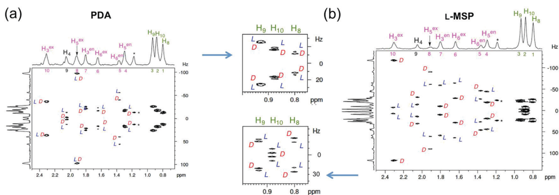
Fig. 2 92.1 MHz NAD- \{^1\text{H}\} Q -resolved Fz 2D spectrum (tilted and symmetrized) of 5 (ee( \nu ) = 30%) in (a) PDA/ \text{CHCl}_3 phase and (b) L -MSP/ \text{CHCl}_3 , showing the assignment of {}^2\text{H} -QDs accordingly to atomic numbering see (figure 2) and the associated stereodescriptors for each pair of {}^2\text{H} -QDs assigned according to the difference of peak intensity between the major ( \nu )- and minor ( L )-enantiomer. In the central panel a magnification of the methyl region is displayed. The peak labelled with an asterisk is assigned to the NAD signal of ethanol added as a stabilizer of \text{CHCl}_3 .
