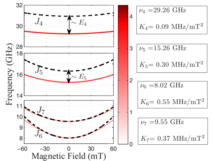
FIG. 5. Numerical color map of the powder ESR absorption intensity as a function of field and frequency in the perpendicular mode for J_4 to J_7 Co 2+ pairs. The dashed line is the analytical resonance field transition obtained from (3).
