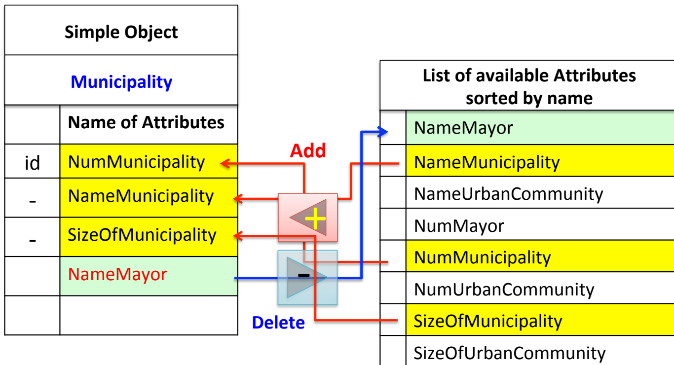
Figure 8. Object type descriptor interface (OTDI).
