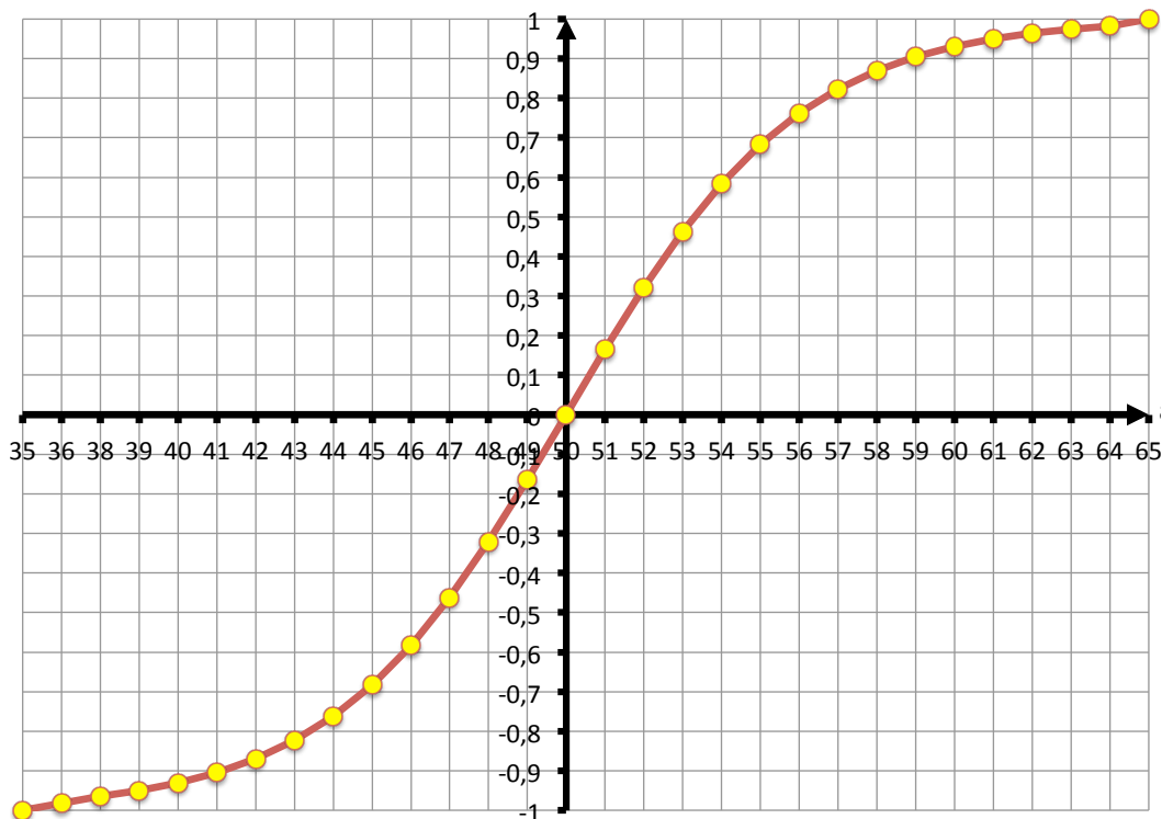
Figure 17. Fuzzy characteristic function μAge(H(x)).
