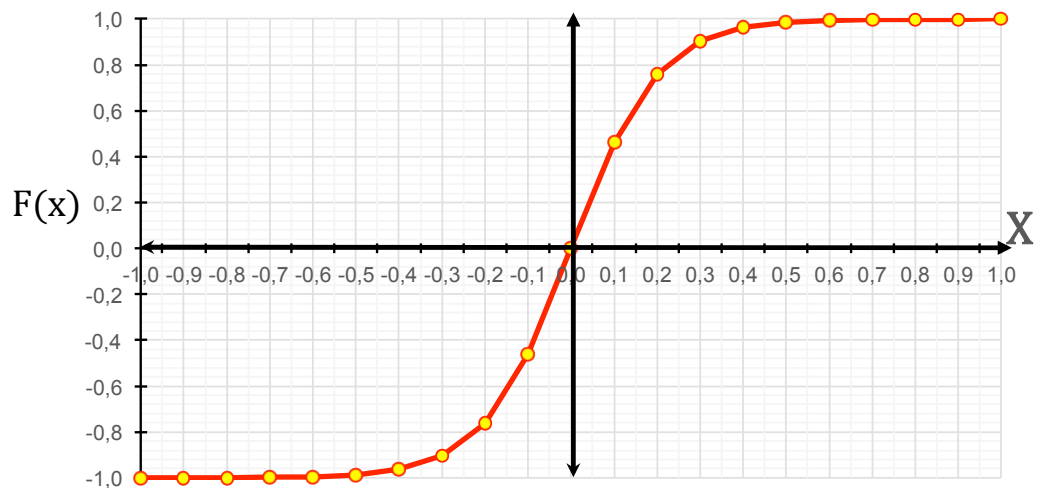
Figure 2. A sigmoid membership function on [-1, 1] \rightarrow [-1, 1] .
