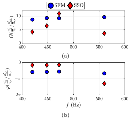
Figure 5: The gain (a) and phase (b) of relative plenum velocity fluctuations to relative chamber velocity fluctuations. At f_0 = 448 Hz ( l_c = 315 mm) and 560 Hz ( l_c = 250 mm), the results are shown when the chamber velocity fluctuations of SFM coincide with those of SSO. At f_0 = 420 Hz ( l_c = 350 mm) and 472 Hz ( l_c = 300 mm), the results are shown when the chamber velocity fluctuations of SFM are closest to SSO.
