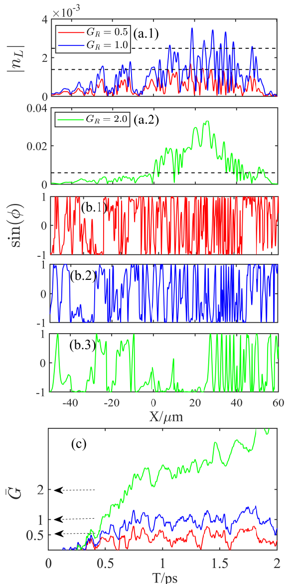
FIG. 7. Red, blue, and green lines represent the cases with G_R = 0.5, 1 and 2 , respectively. Shown are in (a) the density perturbations |n_L| as a function of space at t=1 ps. The horizontal black dashed lines indicate the solution to Eq. (25); in (b) \sin \phi of the relative phase \phi = \phi_0 - \phi_1 - \phi_L as a function of x at t=1 ps; in (c) the instantaneous effective gain \bar{G} value defined in Eq.(24) as a function of time in ps. All simulation results shown are from a single realisation.
