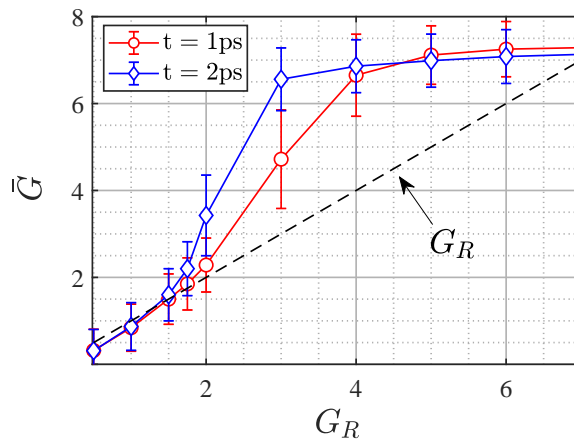
FIG. 6. Effective gain \bar{G} of SRS backscatter as a function of the Rosenbluth gain G_R (expected without SRS destabilization), here, in contrast to Fig. 5, for the case with an incoherent, large bandwidth seed for the incoming scattered light. Black dashed line: \bar{G} = G_R as guide line, red circular and blue diamond markers show simulation data at times t = 1\text{ps} and 2\text{ps} , respectively, with error bars from standard deviation.
