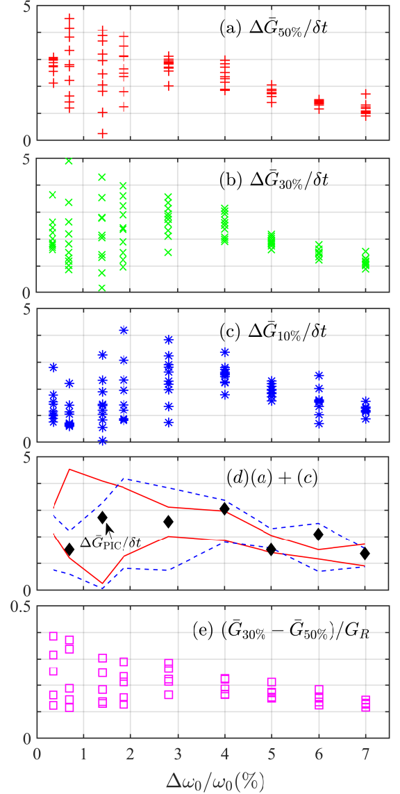
FIG. 17. Numerical evaluation of the temporal increment \Delta \bar{G}_p/\delta t in units of \text{ps}^{-1} from Eq. (35) as a function of the relative bandwidth \Delta\omega_0/\omega_0 shown for complementary probabilities p = F_c(\bar{G}) at (a) p = 50\% , (b) = 30\% and (c) = 10\% . For each bandwidth value, 10 simulation data points computed from Eq. (35) are shown. Subplot (d) shows the envelopes following the outermost data points from (a)-(c); indicating the value of \Delta \bar{G}_p/\delta t attained with up to 10% (upper) and up to 90% (lower bound) probability, respectively. Black symbols: PIC results from single realisations. The evolution of \Delta \bar{G}_p/\delta t for 30% and 50% are difficult to distinguish in subplots (a) and (b). Therefore we show in (e) the difference between \bar{G}_{30\%} and \bar{G}_{50\%} divided by G_R .
