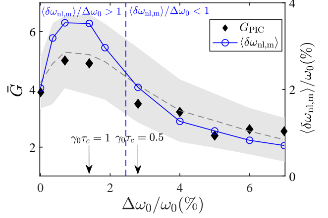
FIG. 15. SRS amplification, in terms of the effective gain value \bar{G} as a function of the relative bandwidth \Delta\omega_0/\omega_0 . The dashed line shows the expectation value \langle \bar{G} \rangle obtained from 3-wave coupling simulations (40 realisations for 10 bandwidth values), taken after t = 1.5 ps of interaction. The shaded area indicates the interval, \langle \bar{G} \rangle \pm \sigma(\bar{G}) inside the standard deviation around \langle \bar{G} \rangle . In addition, black symbols show single realization from PIC simulations. Furthermore, the blue line with data points indicates the average maximum kinetic frequency shift \langle \delta\omega_{\text{nl,m}} \rangle (normalized by \omega_0 ) from 3-wave-coupling simulations over 40 realisations (right vertical axis).
