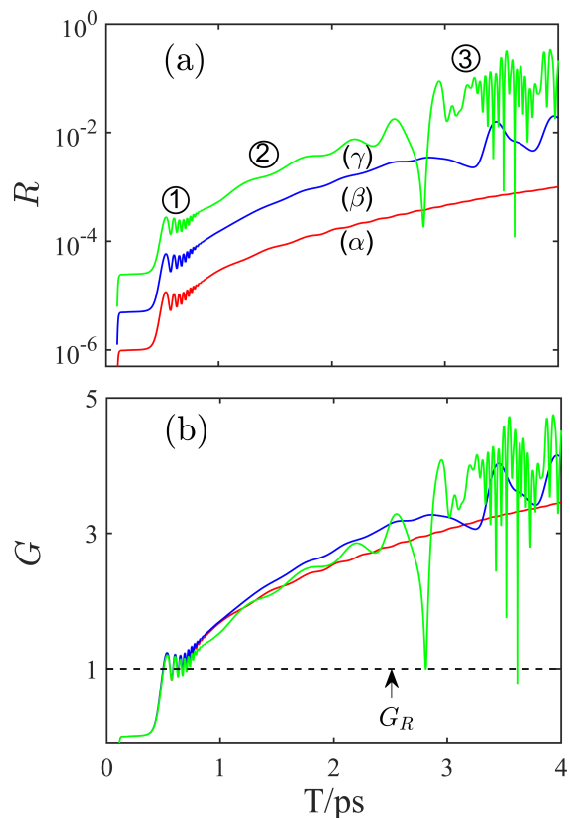
FIG. 5. (a) Instantaneous reflectivity R versus time for different seed intensities: ( \alpha ): I_{sr}/5 , ( \beta ): I_{sr} , and ( \gamma ): 5I_{sr} . Curve \gamma presents the three amplification stages: ① corresponds to fast growth up to 0.5ps and stabilization (Rosenbluth amplification); ② exhibits the destabilization of kinetic effects, the weak nonlinear stage of AR; ③ SRS is further destabilized by the kinetic effects after upper limit of AR is reached, resulting in the further amplification and modulation; (b) Instantaneous amplification factor G(t) for these three different seed intensities.
