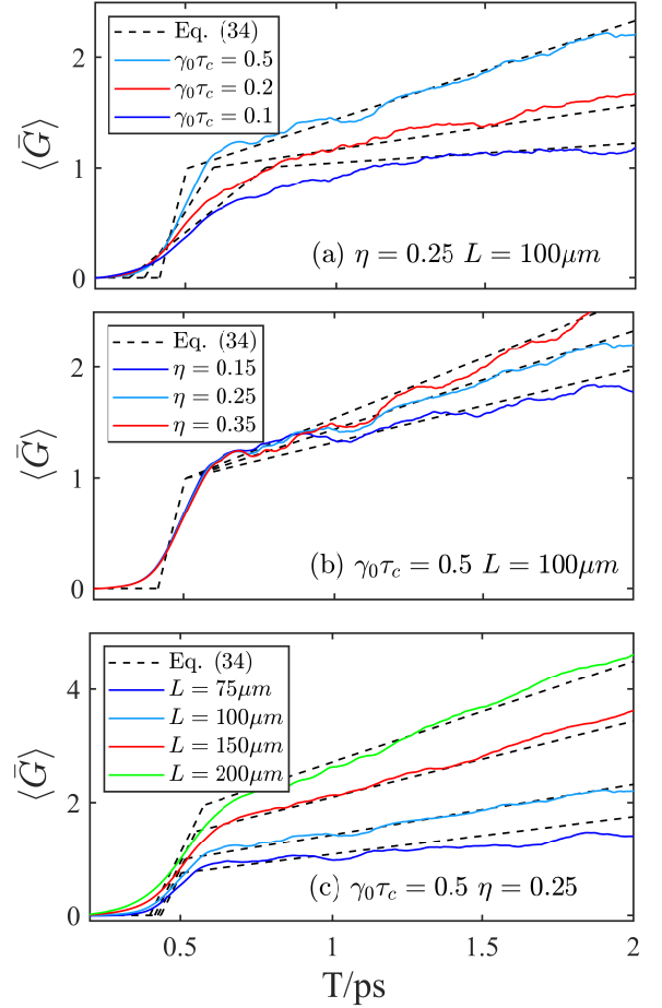
FIG. 13. Evolution of average effective gain \langle \bar{G} \rangle versus time obtained from simulations: (a) for different \gamma_0 \tau_c values with \eta = 0.25 and L = 100\mu m ; (b) For different \eta values with \gamma_0 \tau_c = 0.5 and L = 100\mu m ; (c) For characteristic length L with \gamma_0 \tau_c = 0.5 , \eta = 0.25 . Dashed black lines indicate the values computed from the model, Eq. (34).
