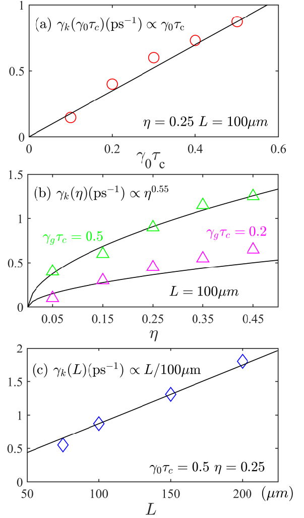
FIG. 12. Growth rate \gamma_k in relation to \gamma_0\tau_c , \eta and L : in (a) as a function \gamma_0\tau_c for fixed values of \eta = 0.25 and the profile gradient length L = 100\mu\text{m} , in (b) as a function of the kinetic factor \eta for fixed values of \gamma_0\tau_c = 0.2 and 0.5 and L = 100\mu\text{m} , and in (c) as a function of the gradient length L for fixed \eta = 0.25 and \gamma_0\tau_c = 0.5 . Markers in different color correspond to numerical simulations, solid lines to the parameter scaling indicated in the legend, i.e., in (a) linear with \propto \gamma_0\tau_c , in (b) \propto \eta^{0.55} , and in (c) linear in L .
