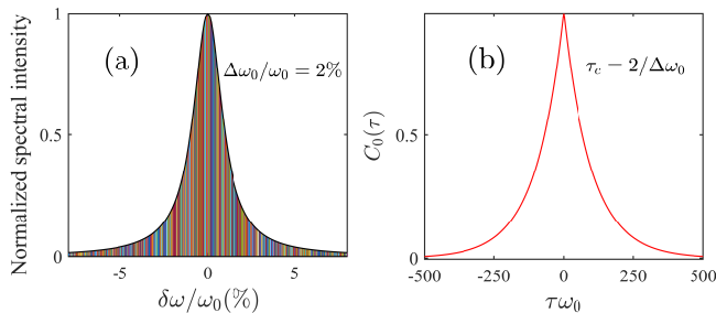
FIG. 18. (a) Intensity spectrum (normalized) with a Lorentzian shape similar to |f|^2 as a function of the deviation \delta\omega from the central frequency \omega_0 for the pump laser I(\delta\omega) , see Eq. (18) in the main text, and (b) the corresponding correlation function C_0(\tau) having the bandwidth \Delta\omega_0/\omega_0 = 2\% .
