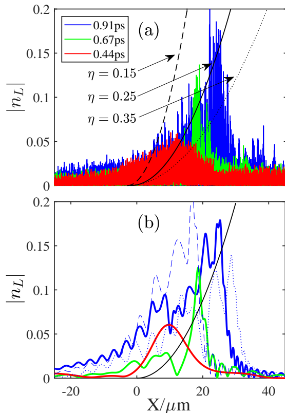
FIG. 3. Spatial profile, in x , of the EPW amplitude taken at three different time instants, t = 0.44, 0.67, and 0.91 \text{ps} , (a) taken from a PIC simulation and (b) taken from solutions of three waves coupling equations, together with the parabola following the solution for AR, Eq. (19), for different values of the parameter \eta : in (b) bold colored lines correspond to \eta = 0.25 , while dashed (dotted) correspond to \eta = 0.15 ( \eta = 0.35 , respectively). Different colors correspond to different time instants as in (a).
