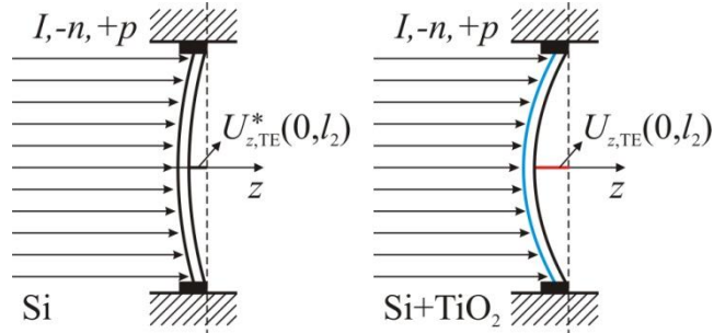
Figure 6. Schemes of the thermoelastic displacement of the irradiated Si membranes with U_{z,TE}(r, z) and without U_{z,TE}^*(r, z) a thin \text{TiO}_2 film (blue line), where photogenerated electrons ( -n ) and holes ( +p ) are present.
