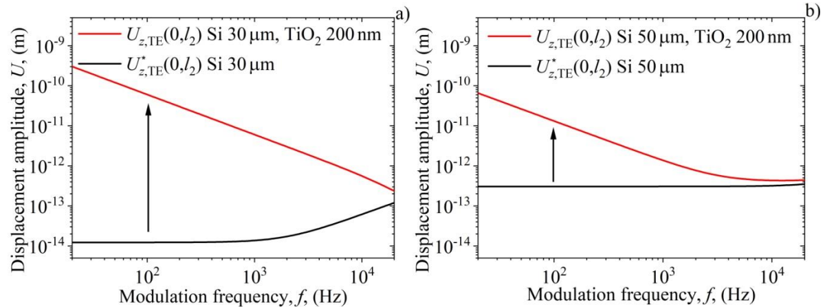
Figure 5. Thermoelastic displacements of the a) 30 \mu\text{m} and b) 50 \mu\text{m} Si membranes with U_{z,\text{TE}}(r,z) and without U_{z,\text{TE}}^*(r,z) a thin TiO 2 film, as functions of modulation frequency f .
