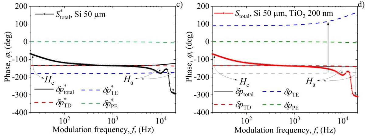
Figure 4. Experimental (asterisks) and corrected (solid line) total photoacoustic signals along with the corresponding signal components (dashed lines) for the phases \varphi of the Si membranes without S_{\text{exp}}^*(f) (a,c) and with S_{\text{exp}}(f) (b,d) a thin TiO 2 film, as functions of the modulation frequency f .
