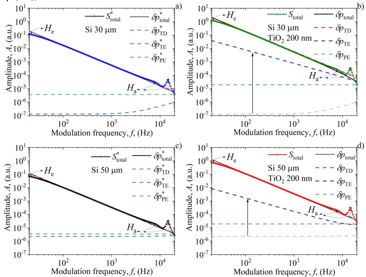
Figure 3. Experimental (asterisks) and corrected (solid line) total photoacoustic signals along with the corresponding components (dashed lines) for the amplitudes A of the Si membranes without S_{\text{exp}}^*(f) (a,c) and with S_{\text{exp}}(f) (b,d) a thin \text{TiO}_2 film, as functions of the modulation frequency f .
