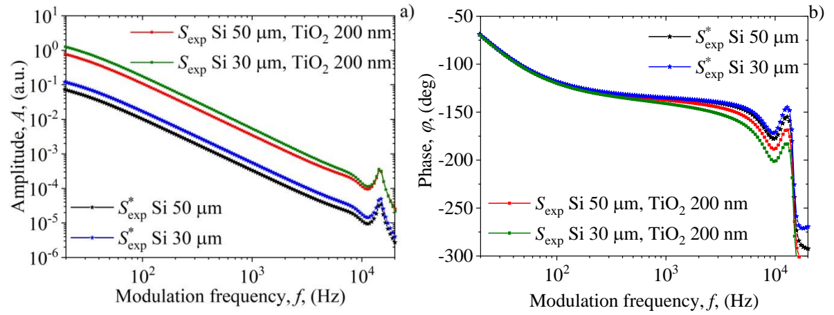
Figure 2. Experimental photoacoustic signal a) amplitude A and b) phase \varphi of Si membranes with S_{\text{exp}}(f) and without S_{\text{exp}}^*(f) thin \text{TiO}_2 film as a function of modulation frequencies f .
