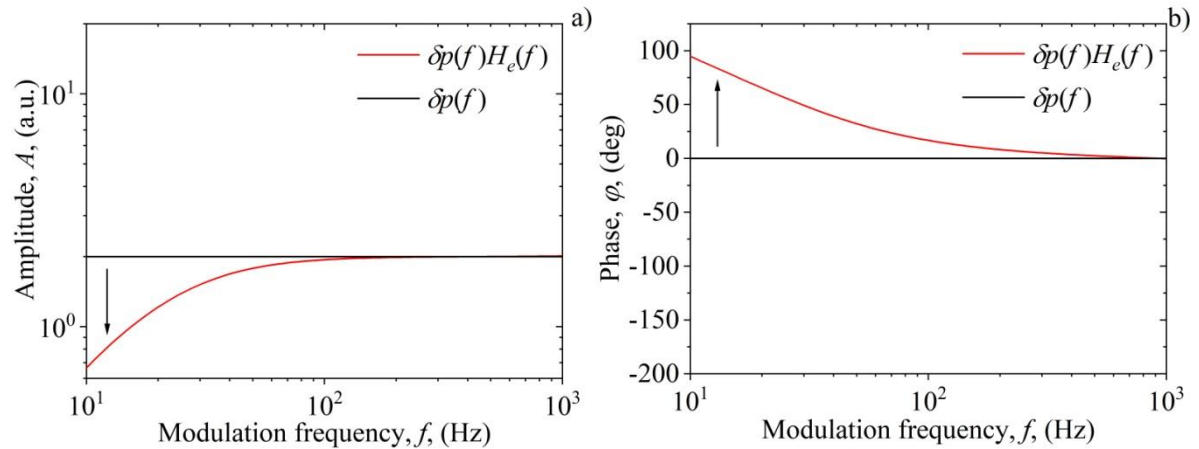
Figure 7. Typical signal distortion (red line) of the a) amplitude A and b) phase \varphi for modulation frequencies f < 1 kHz.
