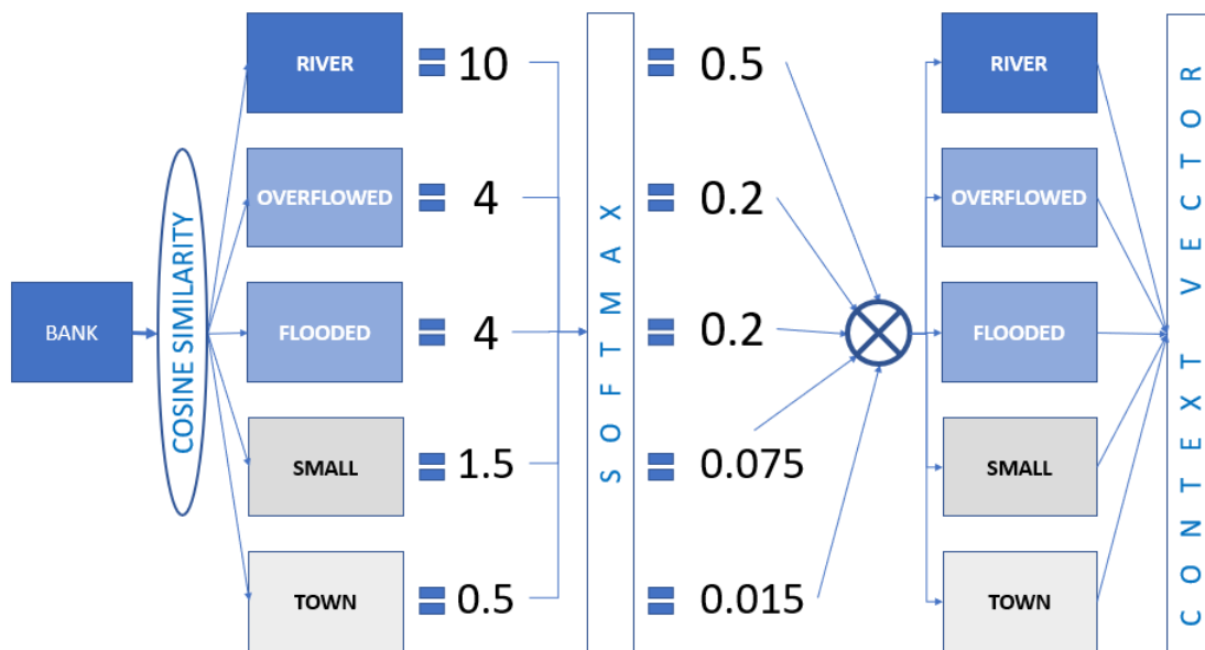
Figure 1: Illustration of the attention mechanism
