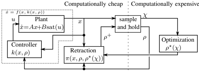
Fig. 1. Main components of the hybrid closed loop (34). The overall system can be split in continuous-time dynamics and discrete-time dynamics. The discrete time update through the optimization problem (19) may be computationally expensive, while the rest of the components are computationally cheap.
