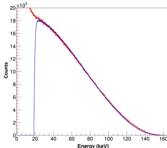
Figure 4. Comparison of measured spectrum (blue) with simulated spectrum (red) ^{14}\text{C} decay (allowed transition).
