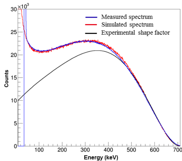
Figure 5. Comparison of measured spectrum (blue) with simulated spectrum (red). The initial spectrum (black) used as input of the simulation comes from an experimental shape factor from Rotzinger et al. [12] of ^{36}\text{Cl} decay (second forbidden non-unique transition).
