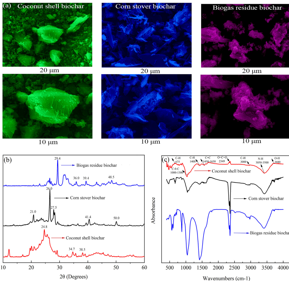
Fig. 1. Analysis of biochars by (a) scanning electron microscopy (SEM), (b) X-Ray diffraction (XRD) and (c) Fourier-transform infrared spectroscopy (FTIR).
