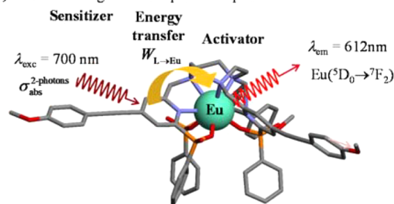
d) TPA occurring in an europium complex
