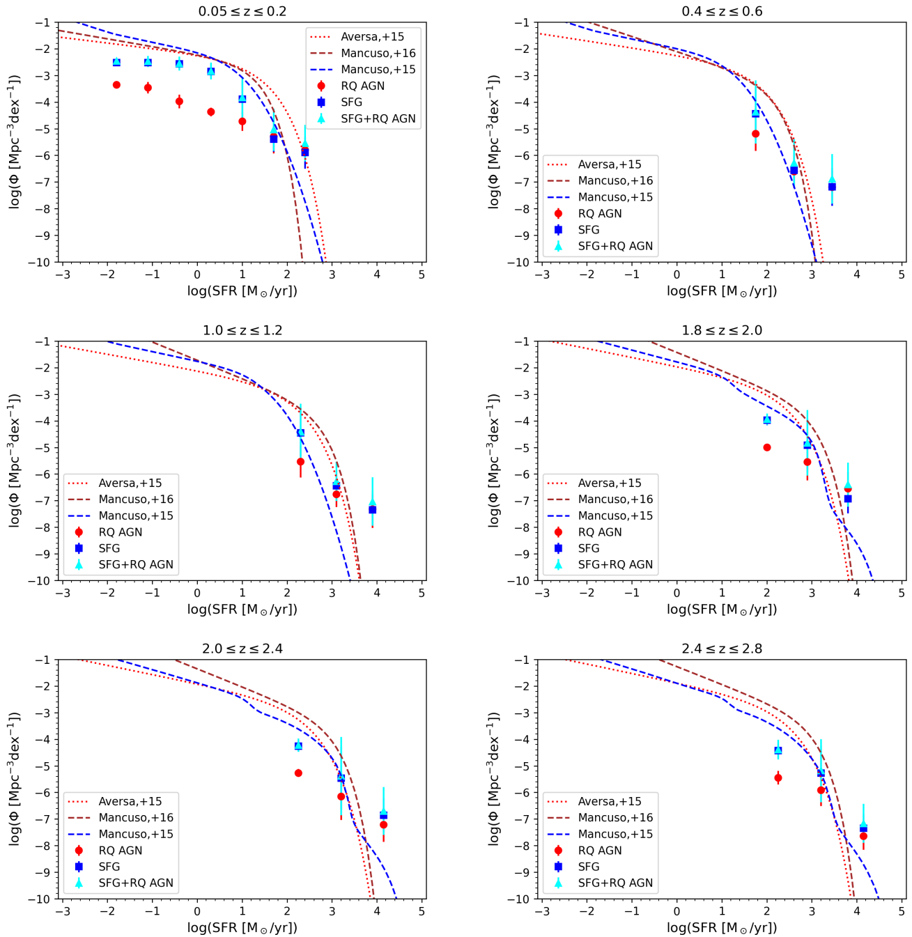
Fig. 9. Comparison of our observational estimates of the SFR functions with the theoretical ones by Mancuso et al. (2015) , Aversa et al. (2015) , and Mancuso et al. (2016) , brown dashed lines). The lines can be seen as representations of observational estimates of the SFR functions based on combinations of classical UV and FIR star-formation tracers (see text). They indicate that the LoTSS data allow us to measure space densities of typical high- z SFGs, with \text{SFR} \sim 100 M_{\odot} \text{yr}^{-1} , up to z \approx 2.5 . The two inflection points, at \log(\text{SFR}/M_{\odot} \text{yr}^{-1}) \approx 1 and \approx 3.5 , of the Mancuso et al. (2015) line for z > 1.5 correspond to the transition from the dominance of late-type galaxies to that of star-forming protospheroids and to the dominance of strongly lensed galaxies, respectively. The error bars are the quadratic sums of Poisson uncertainties and of sample variance; they are generally smaller than the symbols. The real uncertainties are much larger, especially at z > 1 where the quality of photometric redshifts increasingly worsens, but difficult to quantify.
