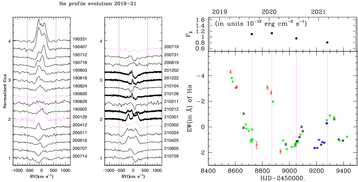
Figure 1. Left-hand panels: Evolution with time of the profile of the H\alpha line observed in HD 119682 during our monitoring campaign. Dates in YYMMDD are provided to the right of the line. Spectra taken close to the time of an XMM-Newton observation are shown with a magenta dotted line, while vertical black dotted lines indicate the interval chosen for EW determination. Note that the noisier ( \text{SNR} < 20 ) or lower resolution ( R < 3000 ) spectra are not shown. Right-hand panel: Evolution with time of the H\alpha EWs measured in the -600 to +600 \text{km s}^{-1} interval and of X-ray fluxes. The top axis provides the date in years, while the bottom axis uses Julian dates. Red open triangles display the values obtained from the noisier spectra ( \text{SNR} < 20 ), black open squares those measured on the lower resolution data ( R < 3000 but \text{SNR} > 20 ), green dots those derived from other amateur spectra ( R > 3000 and \text{SNR} > 20 ), and blue symbols those measured on ESO spectra (stars for UVES and open pentagon for X-Shooter). Note the very good agreement between ESO and amateur data taken at similar dates. The vertical magenta dotted lines indicate the times of the XMM-Newton observations.
