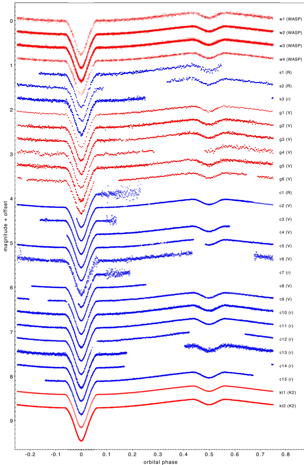
Figure 1. The 30 light curves of HW Vir analysed in this study, plotted as a function of the orbital phase. Each curve is labelled with an identifier (matching those in Table 2) and the filter name (uppercase for the Bessel system, lowercase for SDSS). The SuperWASP (w1–w4) and K2 (kt1–kt2) curves are split into separate chunks as described in Section 3. The colour scheme is used for visual reference to identify each set of light curves.
