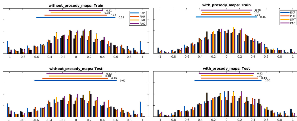
Fig. 12. Automatic assessment: distribution of prediction errors for training (top) vs. test (bottom) partitions, without (left) vs. with (right) taking prosodic features into account distributions for the 4 subjective dimensions are superimposed. Standard deviations are also superimposed with horizontal bars. As expected, significant reduction of variance is achieved for phrasing (PHR) and expressivity (EXP) when taking prosody into account.
