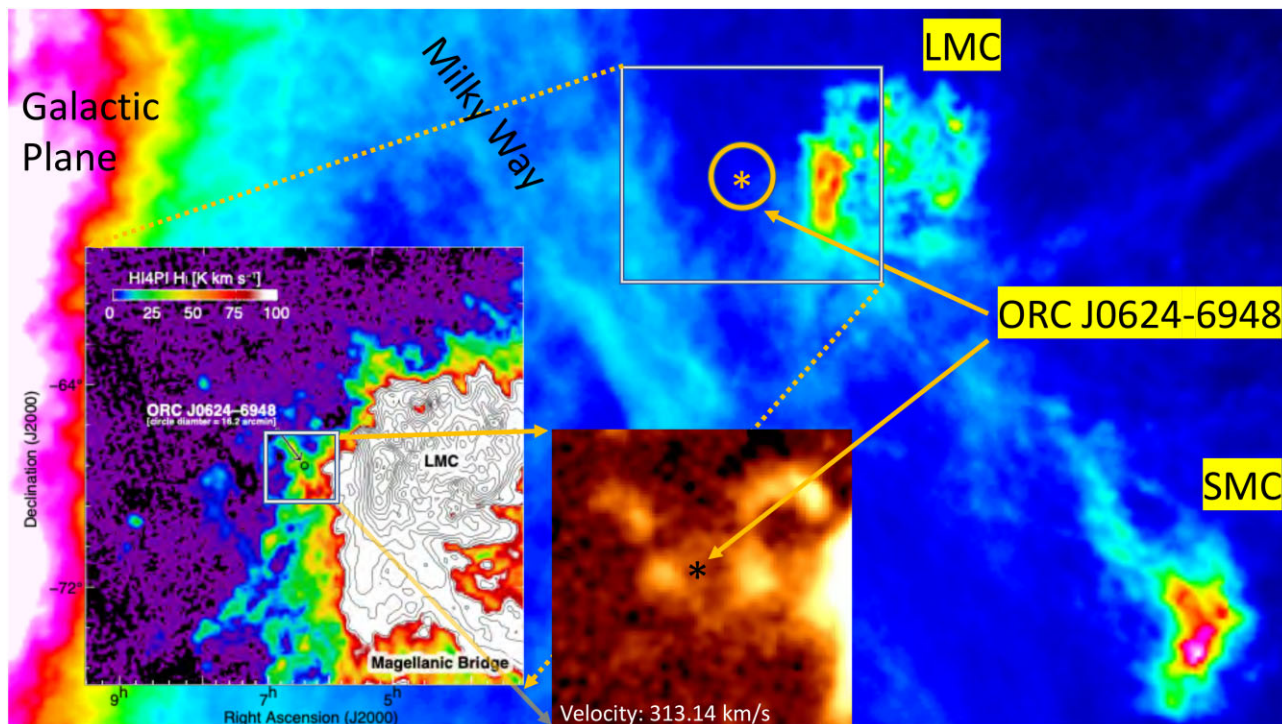
Figure 9. The Parkes GASS and HIPI (insets) H I images indicating the position of J0624–6948 with respect to the LMC, SMC, and MW. The image beam size is 16.2 arcmin. In the leftmost inset, the integrated velocity range is from v=189.5 to v=319.6 \text{km s}^{-1} . The contour levels are 100, 150, 250, 400, 600, 850, 1150, 1500, 1900, 2350, and 2800 \text{K km s}^{-1} .
