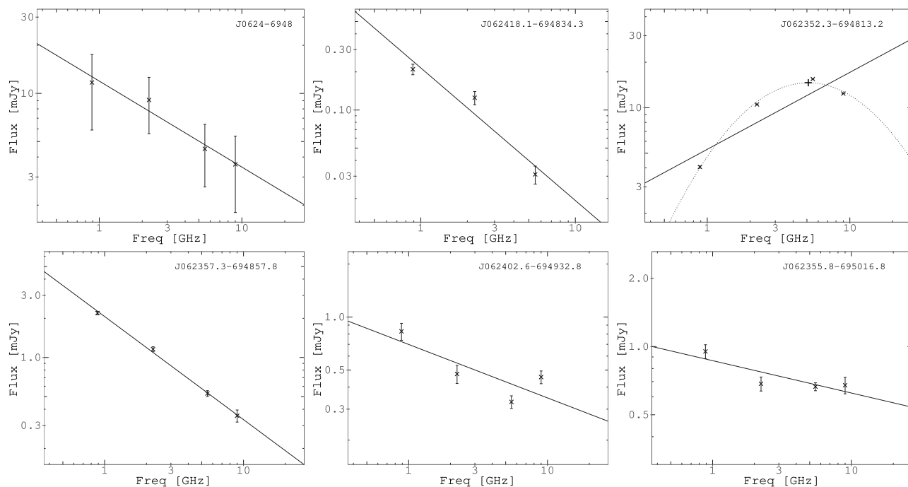
Figure 8. Spectral index plots for J0624–6948 (top left), central source (top middle), and four bright sources near south-west from J0624–6948. See Table 2 for more details. The plus (+) sign in the top right image indicates the turnover frequency at \sim 4900 MHz for the GPS source ASKAP J062352.3–694813.2.
