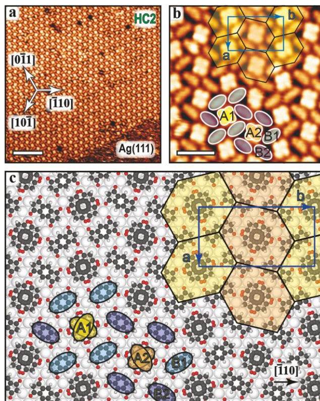
Figure 3: (a,b) STM images of the self-accommodating honeycomb supramolecular phase HC2 formed by INDO 4 on Ag(111). (c) Corresponding adsorption model. Ag surface atoms are represented as light grey spheres. Scale bars: (a) 8 nm, (b) 2 nm.
