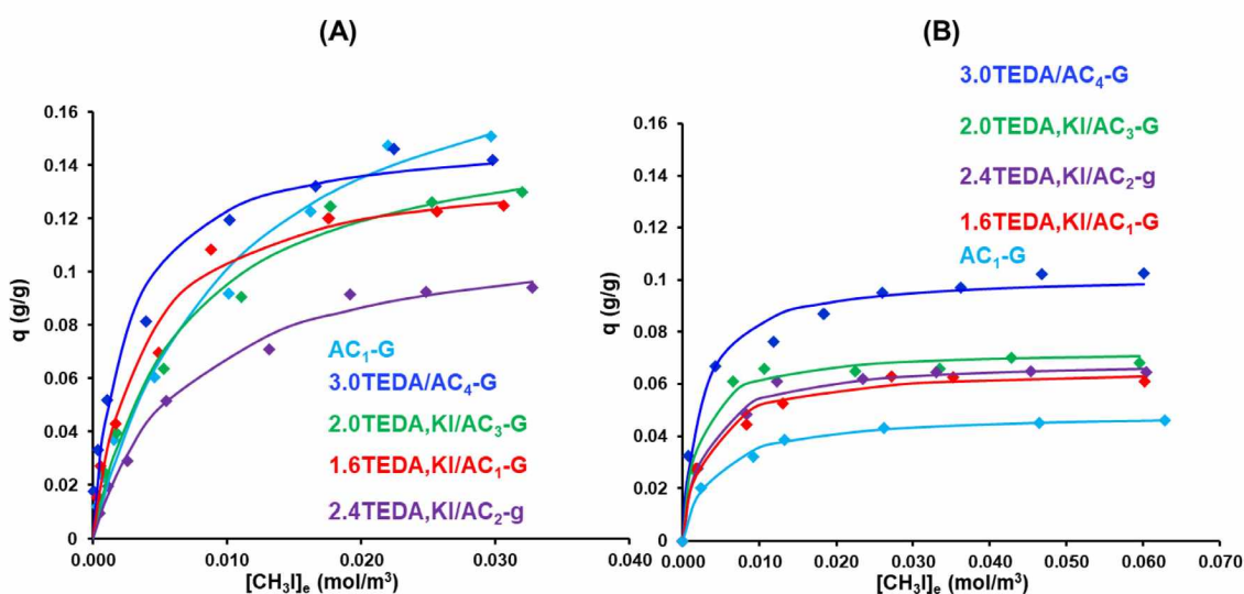
Fig. 4.. Experimental CH_3I adsorption isotherms and Langmuir fitted models obtained with the studied activated carbons for the two investigated configurations: (A) normal operating conditions; (B) severe conditions.
