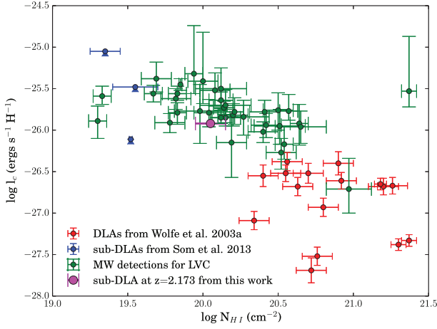
Figure 17. Cooling rate per H atom, I_c inferred from C\text{II}^* column density, versus H\text{I} column density. The red points denote the sample of QSO DLAs in Wolfe et al. (2003). The green points represent the measurements for low-velocity interstellar H\text{I} clouds in the Milky Way compiled in Lehner et al. (2004). The point in magenta represents a sub-DLA at z = 2.173 along the sightline to J1106–1731 from this work. The blue points denote the lower limits for the sub-DLAs from Som et al. (2013).
