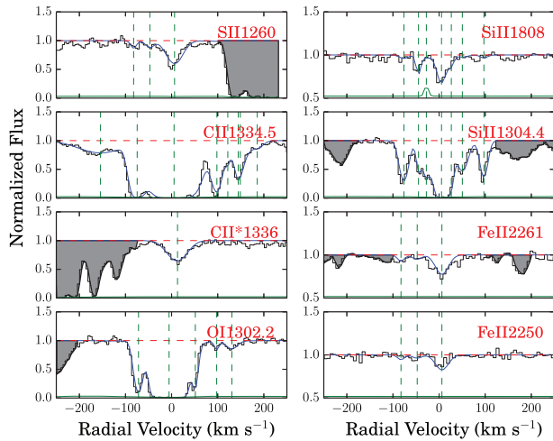
Figure 2. Plots showing Voigt profile fits for metal lines for the sub-DLA at z = 2.173 towards J1106–1731. In each panel, observed data are shown in black, the solid curve in blue shows the fitted profile, and the continuum level is represented by the horizontal dashed line in red. The vertical dashed lines in green are centred at the different velocity components, and the green line at the bottom of each panel shows the 1\sigma error in the continuum-normalized flux. The regions shaded in grey are caused by either telluric absorption or absorption from other systems not associated with the sub-DLA.
