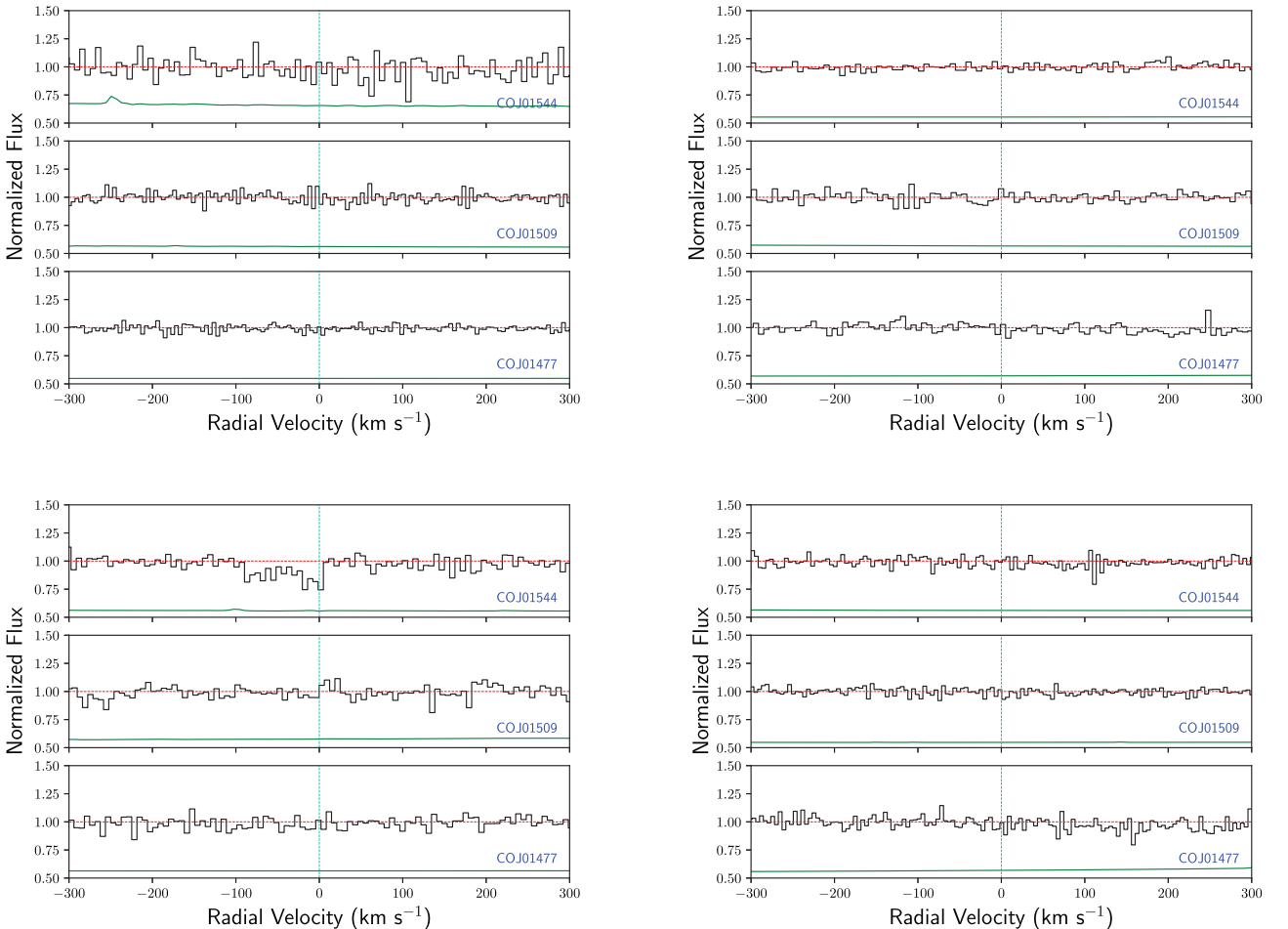
Figure 18. Plot showing the positions of molecular lines of CO for all of the absorbers. The top two plots represent systems at z = 2.173 (left-hand panels) and 2.539 (right-hand panels), and the bottom two plots represent systems at z = 2.635 (left-hand panels) and 2.236 (right-hand panels), respectively.
