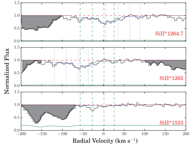
Figure 8. Velocity plots for Si II* \lambda 1264.7, Si II* \lambda 1265, and Si II* \lambda 1533 lines for the absorber at z = 2.236 in the sightline to J1614+1448. The vertical dashed lines in green show the different velocity components included in the profile fits. The dotted lines in blue in the upper panel show the components corresponding to Si II* \lambda 1265, and the dotted lines in blue in the middle panel show the components corresponding to Si II* \lambda 1264.7. The absorption in the shaded regions are not associated with our system.
