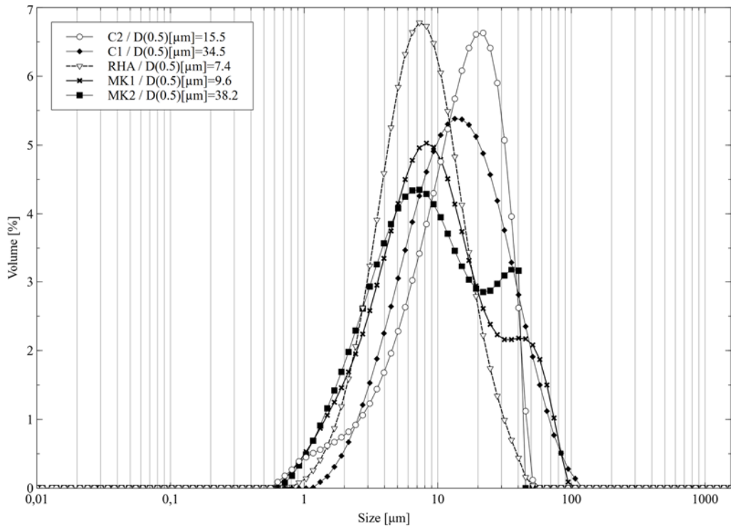
Figure 3: Granulometric curves of the addition materials obtained from the granulometer
