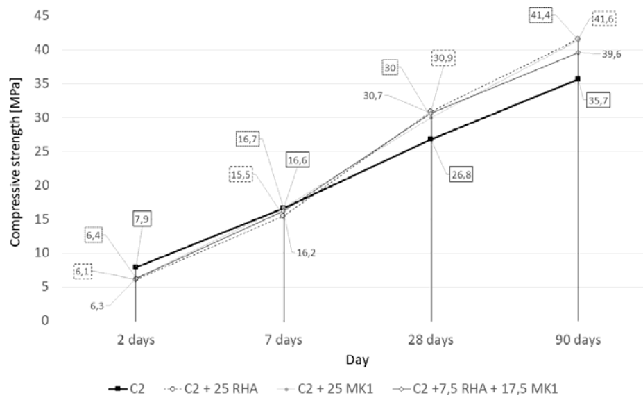
Figure 11: Compressive strength of compositions studied with C2 cement
