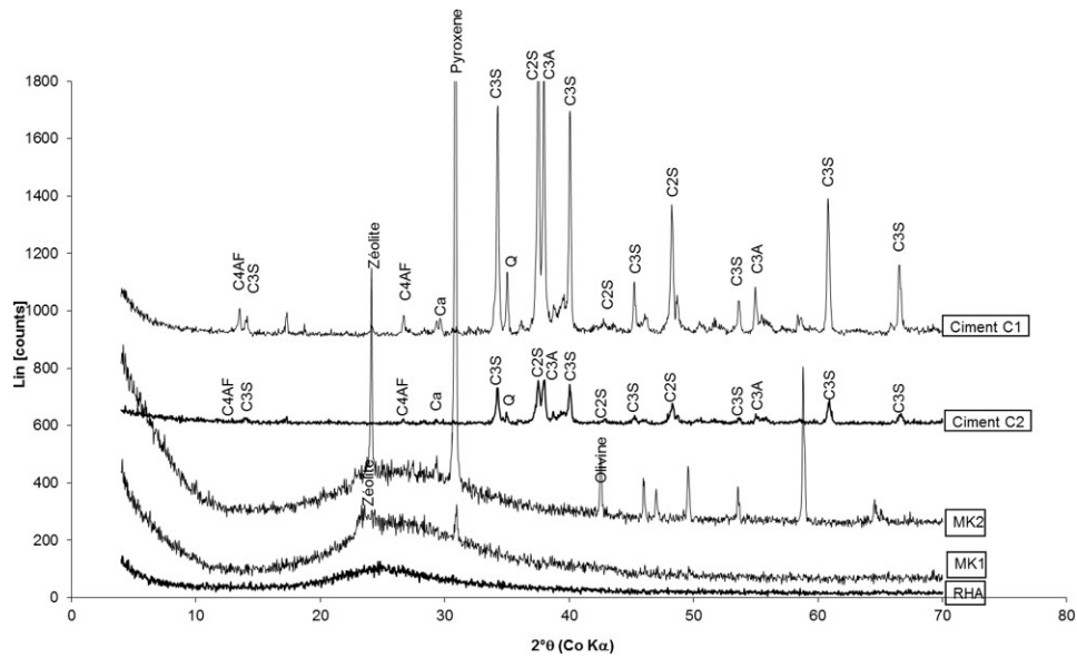
Figure 6: Diffractogram of materials
