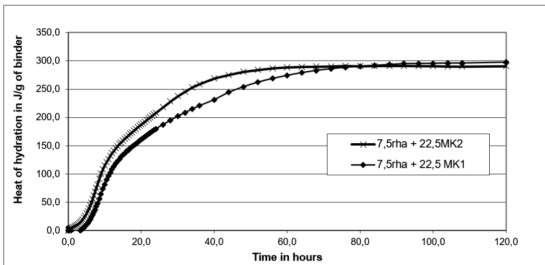
Figure 8: Hydration heat of C1 + 7.5RHA + 22.5MK1/22.5MK2 mixture
