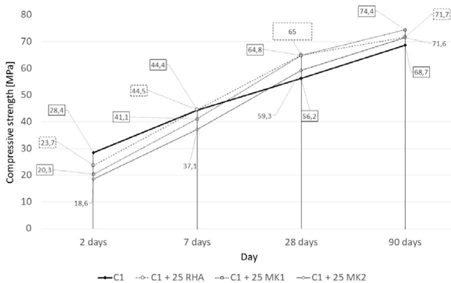
Figure 10: Compressive strength of compositions studied with C1 cement
