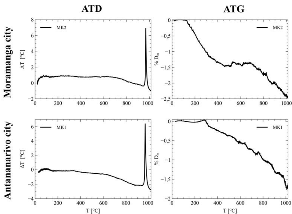
Figure 5: ATD/ATG curves
