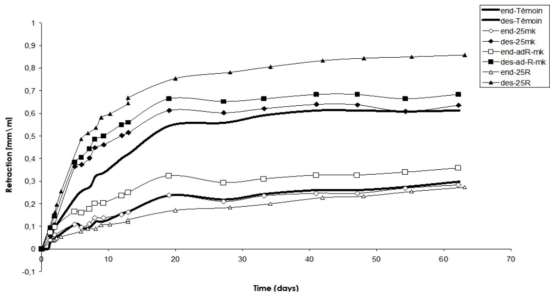
Figure 12: Endogenous retraction and desiccation of components
