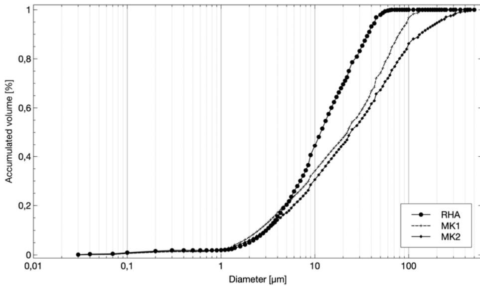
Figure 4: Particle size curve of addition materials
