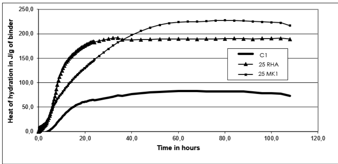
Figure 9: Hydration heat of C1 + 25 mixtures RHA/25MK1 mixture
