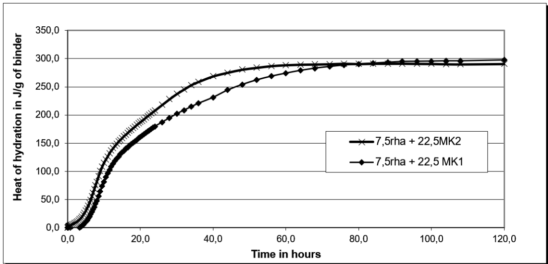
Figure 8: Hydration heat of C1 + 7.5RHA + 22.5MK1/22.5MK2 mixture
